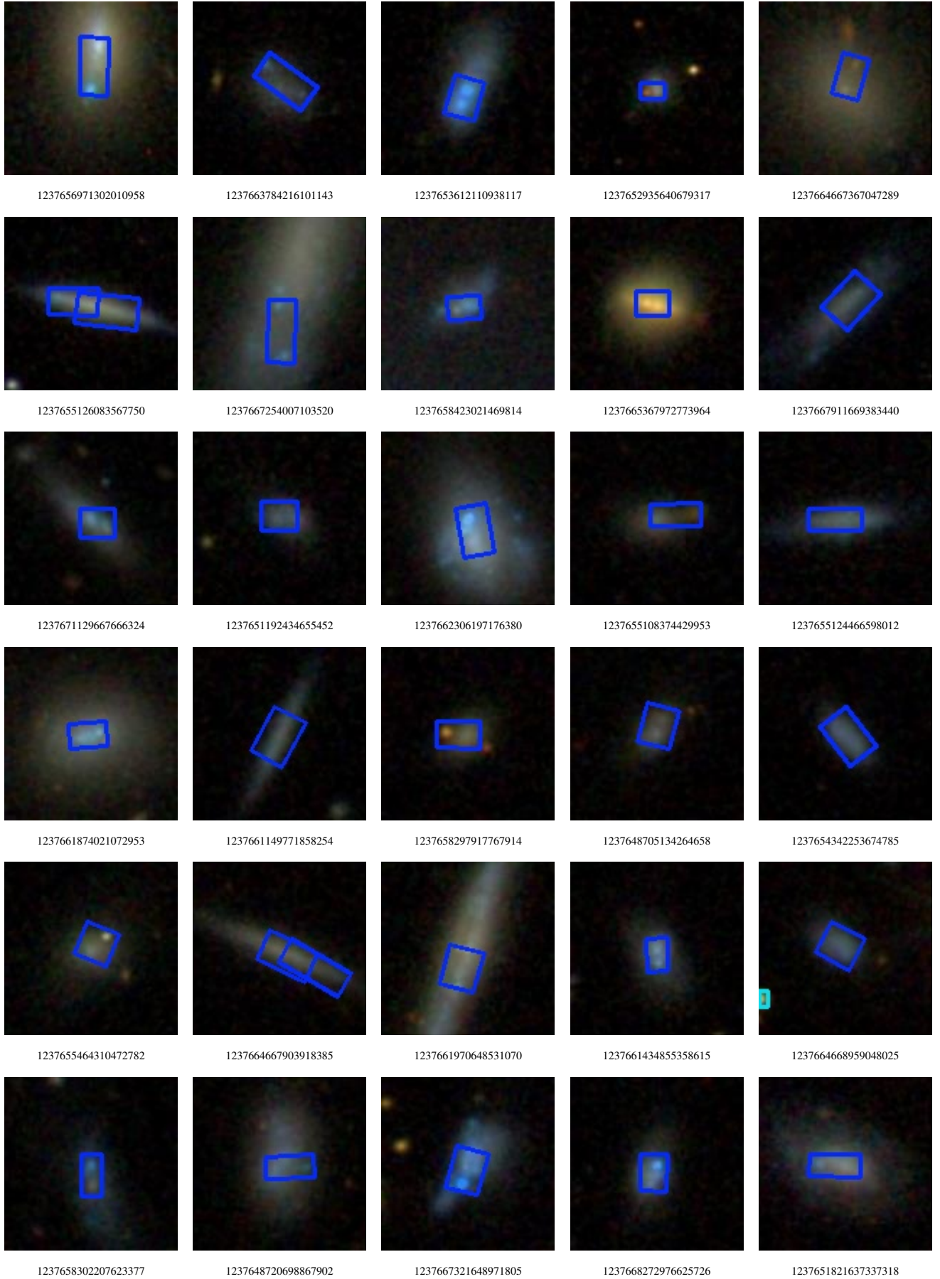
Figure 2. SDSS image cutouts of the sub-kiloparsec dual-nucleus candidates (Fig. 1, continued).
