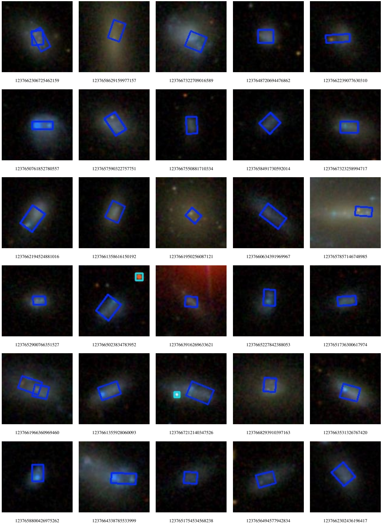
Figure 5. SDSS image cutouts of the sub-kiloparsec dual-nucleus candidates (Fig. 1, continued). MNRAS 000 , 000–000 (2026)
