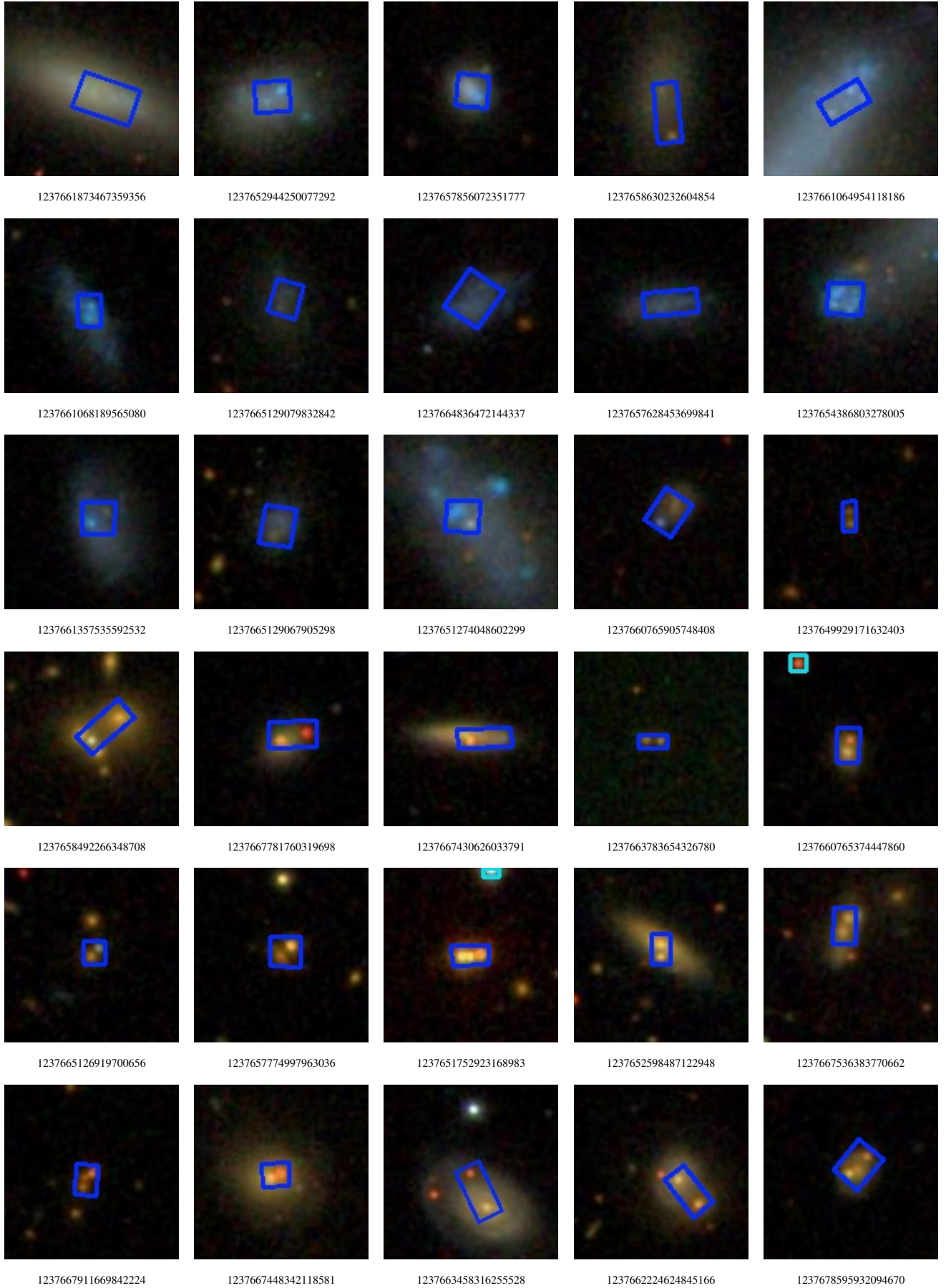
MNRAS 000 , 000–000 (2026) Figure 6. SDSS image cutouts of the sub-kiloparsec dual-nucleus candidates (Fig. 1, continued).
