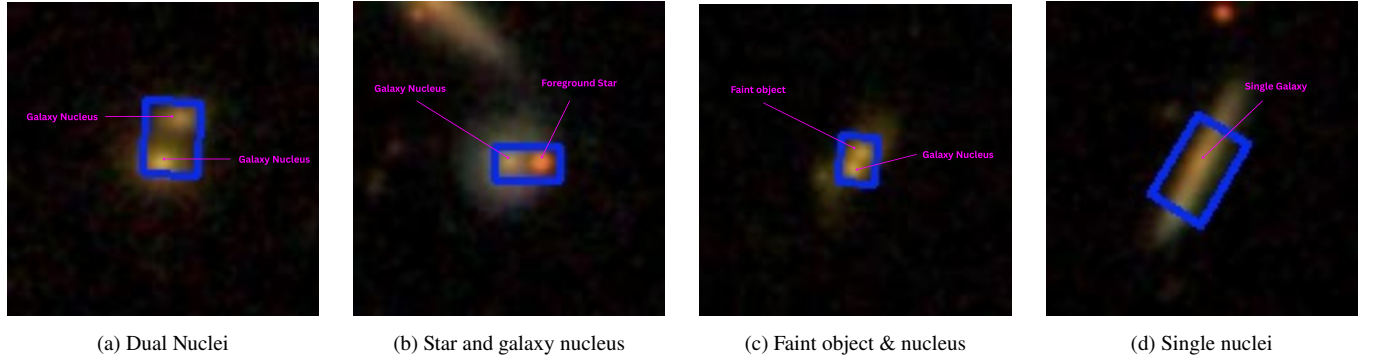
Figure 2. Examples of the four cases encountered in the 29,605 detections. 2a (objID: 1237649962452779114) is Dual Nuclei Detection, 2b (objID: 1237650371020193968) is Foreground Star Detection, 2c (objID: 1237655498126917883) is Faint Object detection, and 2d (objID: 1237648722836062301) is Single Nucleus misclassification. Each panel is a 120 \times 120 pixel SDSS cutout at 0.3'' \text{ pixel}^{-1} , spanning 36'' \times 36'' on the sky.
