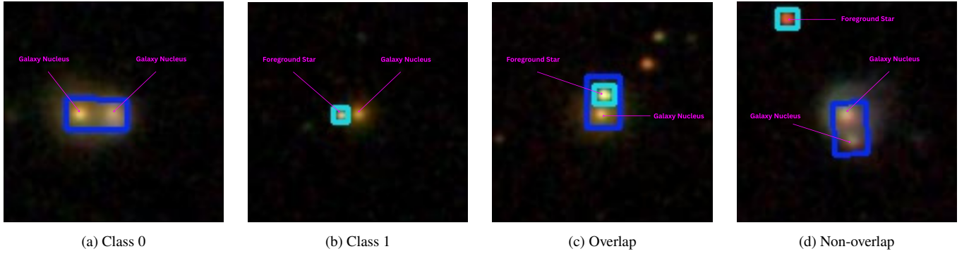
Figure 4. Representative detection outcomes. From left to right: dual nuclei (objID: 1237648702973018278), foreground star (objID: 1237648674533934097), overlapping detections (objID: 1237648674534130384), and non-overlapping detections (objID: 1237648703506022589). Each panel is a 120 \times 120 pixel SDSS cutout at 0.3'' \text{ pixel}^{-1} , spanning 36'' \times 36'' on the sky.
