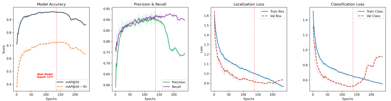
Figure 3. Training evolution of the final YOLOv11x-OBb model. Validation mAP, precision, recall, and loss terms are shown as functions of epoch. The vertical dashed line marks the selected best checkpoint (epoch 137).
