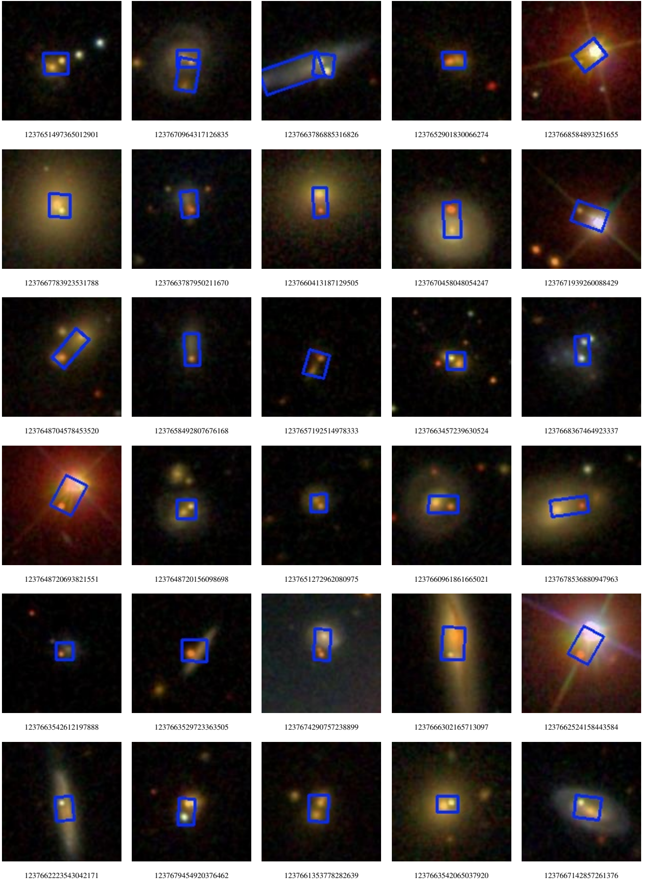
Figure 7. SDSS image cutouts of the sub-kiloparsec dual-nucleus candidates (Fig. 1, continued). MNRAS 000 , 000–000 (2026)
