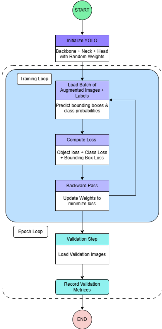
Figure A1. Schematic representation of the YOLO training and validation cycle. Each epoch consists of repeated forward and backward passes over augmented mini-batches, followed by validation evaluation.
