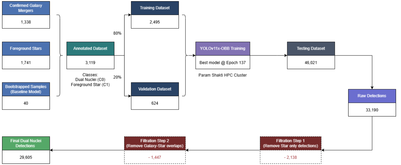
Figure 1. Training and inference pipeline of the final YOLO model. Annotated samples are used for supervised training, followed by large-scale inference and post-processing to construct the final dual-nuclei catalog.
