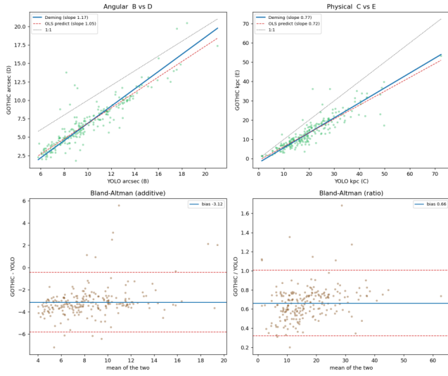
Figure F1. Top: GOTHC versus YOLO with the Deming relationship (solid), the OLS prediction line (dashed) and the 1:1 line (dotted); the Deming line sits above OLS, visualising the attenuation. Bottom: Bland–Altman agreement — additive for the angular pair (left) and ratio for the physical pair (right), with the bias (solid) and 95% limits of agreement (dashed).
