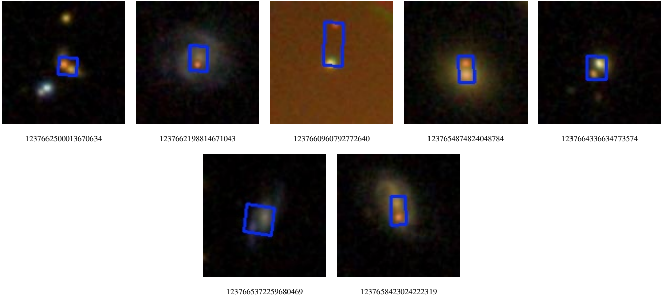
Figure 8. SDSS image cutouts of the sub-kiloparsec dual-nucleus candidates (Fig. 1, continued).
