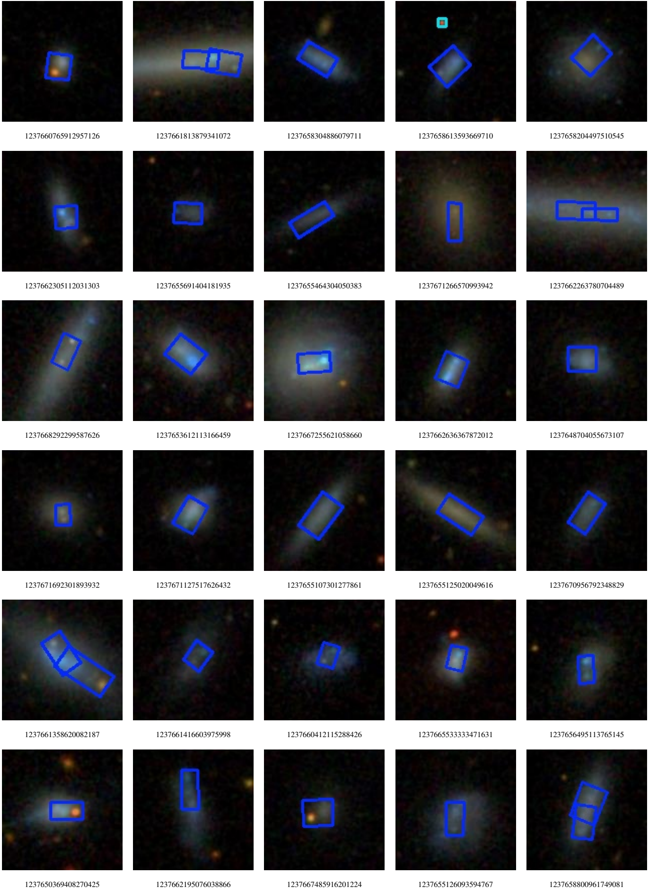
Figure 3. SDSS image cutouts of the sub-kiloparsec dual-nucleus candidates (Fig. 1, continued). MNRAS 000 , 000–000 (2026)
