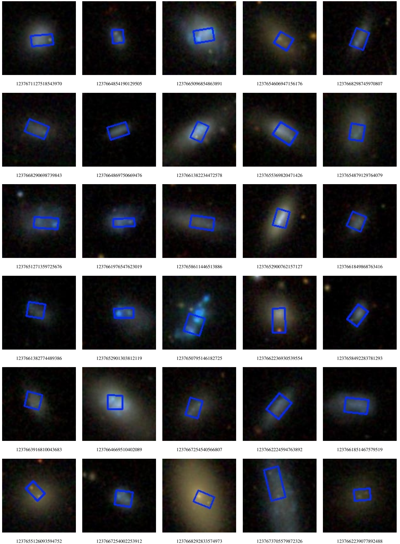
Figure 4. SDSS image cutouts of the sub-kiloparsec dual-nucleus candidates (Fig. 1, continued).
