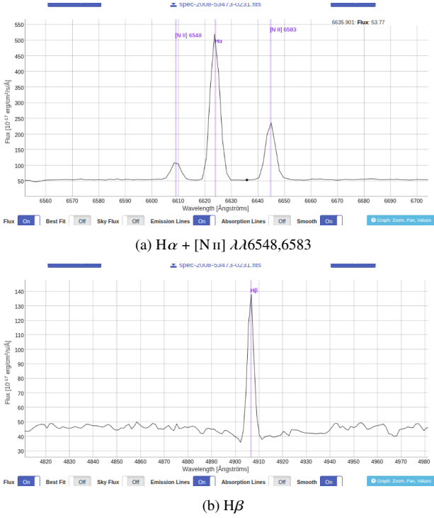
Figure 9. SDSS single-fibre spectrum of objID 1237665367972773964 ( z \approx 0.009 ), the only clearly emission-line system in the \leq 1 kpc subset. Panel a shows the narrow H\alpha line and the [N II] \lambda\lambda 6548, 6583 doublet; panel b shows the narrow H\beta line. Both Balmer lines are single-peaked at SDSS resolution, showing no resolved velocity splitting that would indicate two distinct narrow-line systems. Emission lines are marked by the SDSS pipeline.
