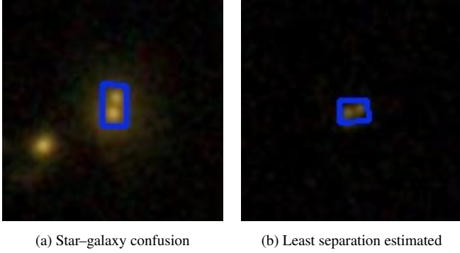
Figure 8. Representative edge cases from the inspected sample. Panel a (objID: 1237651251505528921) shows a foreground star whose profile mimics a galaxy nucleus. Panel b (objID: 1237660239778021761) is the most compact detection in the 400-system inspected sample, with a YOLO OBB-edge separation of \sim 4.61'' , corresponding to a calibrated centroid-to-centroid separation of \sim 0.56'' (Equation 2).
