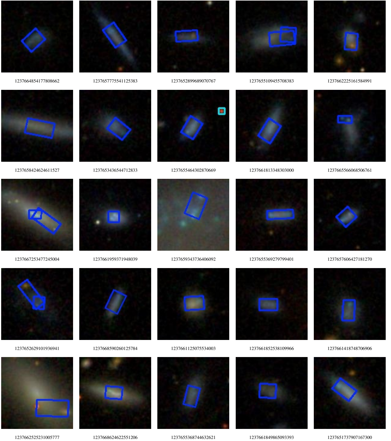
Figure 1. SDSS colour-composite image cutouts of the 212 sub-kiloparsec dual-nucleus candidates ( s_{\text{GOTHIC}} \leq 1 kpc) listed in Table 1, shown in the same order. Each panel is a 120 \times 120 -pixel cutout ( 0.3'' \text{ pixel}^{-1} ; 36'' \times 36'' on the sky) labelled by its SDSS objID. At these separations the two nuclei are unresolved in SDSS imaging (Section 4.3).
