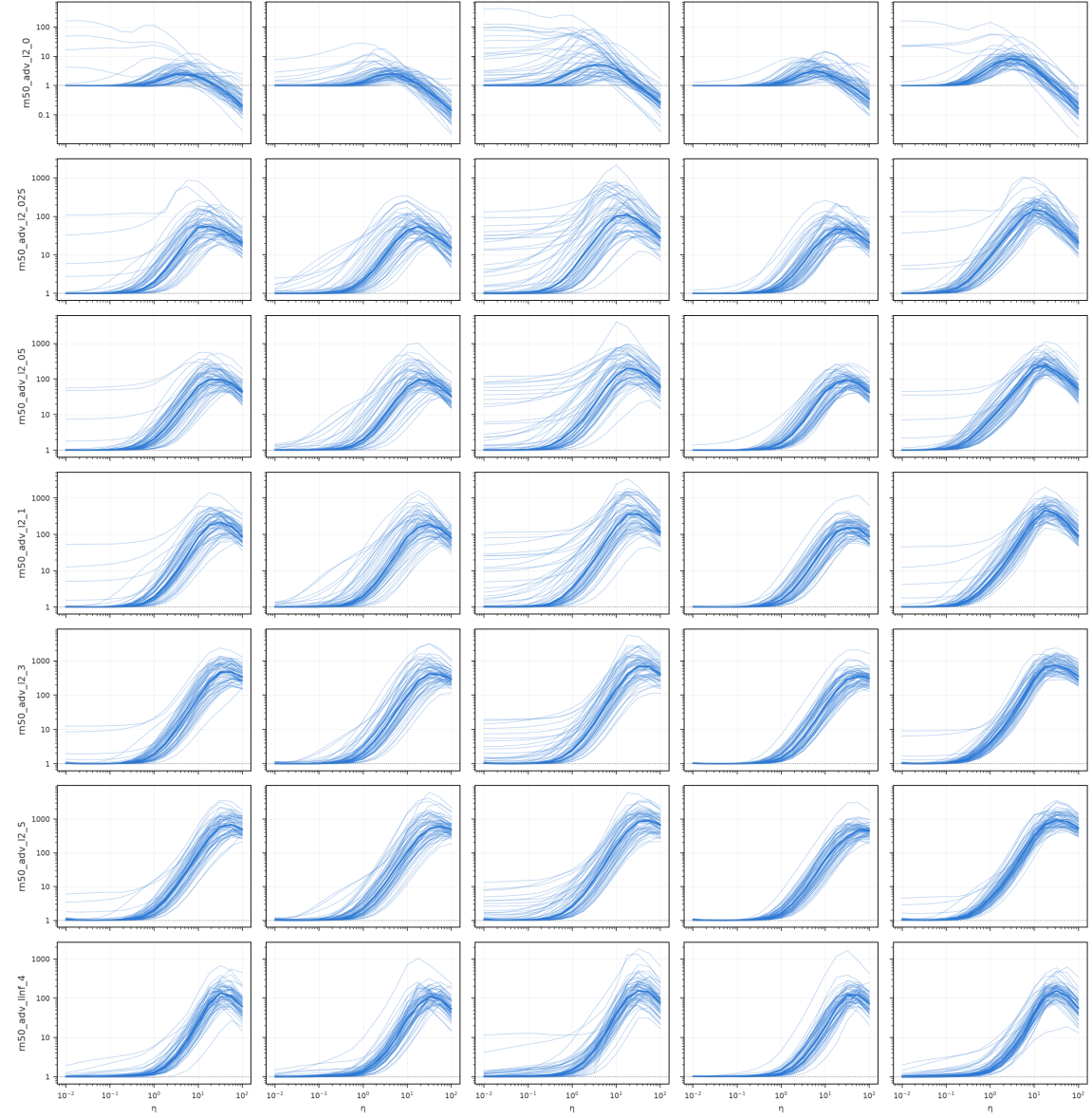
Figure 5: Per-image response profiles for the adversarially trained ResNet-50 family. With increasing training budget \varepsilon , the peak moves to larger \eta and grows; the baseline \varepsilon = 0 retains a peak at small scale.
