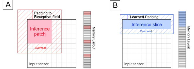
Fig. 2. Proposed slicing vs classical PPBI. Our learned padding results in significantly lower overhead than padding to the full receptive field. Moreover, for NHWC tensor inference, the proposed method relies on data stored in a single continuous memory area, thereby optimizing cache usage.
