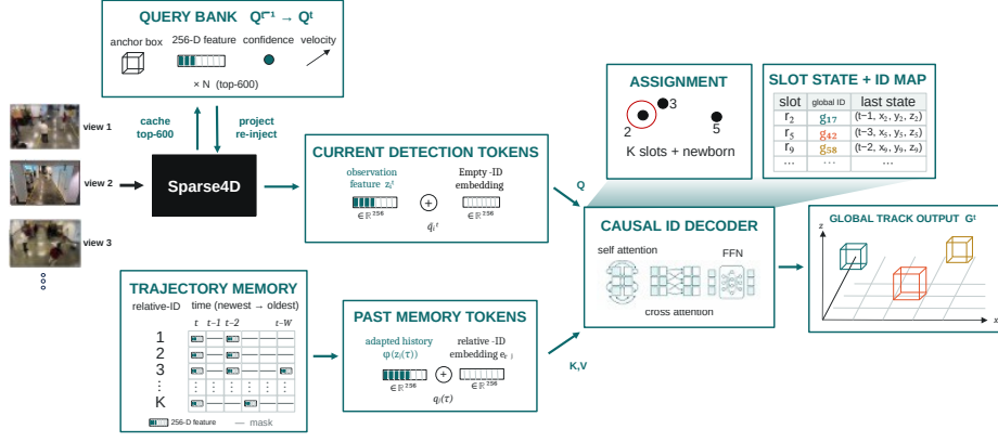
Fig. 2: Architecture details. The recurrent detector fuses all calibrated views with query bank \mathcal{Q}^{t-1} to produce world-frame observations and \mathcal{Q}^t . Detections query the finite trajectory memory \mathcal{M}^{t-1} for relative identities. Geometric masking, discrete assignment, newborn handling, and the MOTIP least-recently-used (LRU) slot lifecycle map those labels through \mu^t to scene-global IDs. Only \mathcal{Q}^t , \mathcal{M}^t , and \mu^t cross the frame boundary.
