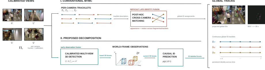
Fig. 1: Difference in multi-camera tracking fusion strategies. Conventional MTMC first forms per-camera tracklets and then performs difficult post-hoc cross-camera fusion. Our decomposition instead fuses calibrated views into one world-frame 3D observation stream before online ID prediction.
