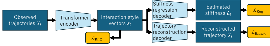
Fig. 2: PRISM architecture. A transformer encoder maps trajectories \mathbf{X}_i to an Interaction Style Vector \mathbf{z}_i , which is structured by RnC loss and decoded for stiffness regression and input reconstruction.
