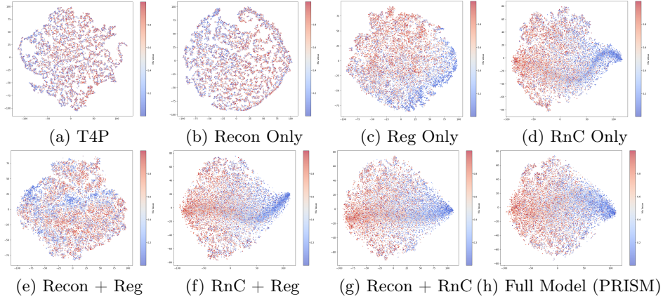
Fig. 3: Latent embedding structure visualized by t-SNE. Embeddings are colored by ground-truth social stiffness \mu ( \mu \approx 0 : aggressive; \mu \approx 1 : cautious). RnC-based configurations show a clearer ordinal gradient than reconstruction- or regression-only variants.
