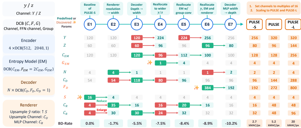
Figure 10: Full agentic evolution process and final parameters at different scales.
