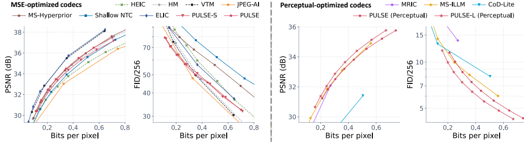
Figure 6: Rate-distortion curves. CLIC Professional validation results for MSE-optimized codecs (left) and perceptually optimized codecs (right). More results are in Appendix C.3.
