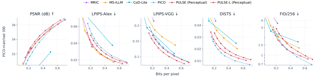
Figure 7: Rate-distortion curves on the 300-image CLIC test subset released by PICO.
