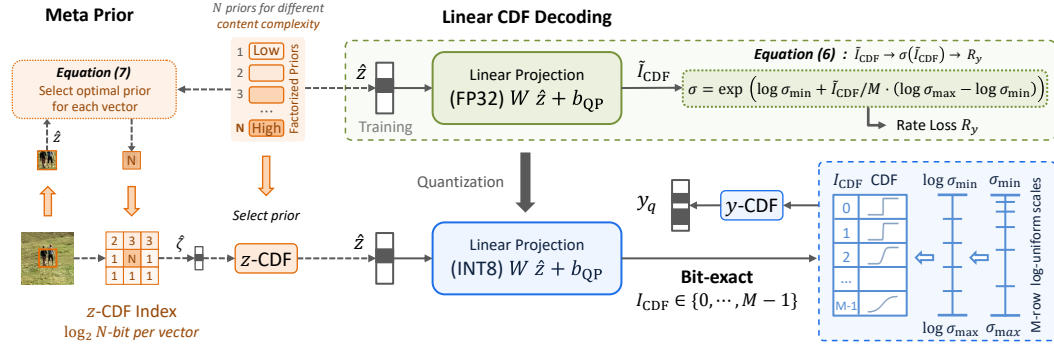
Figure 3: Bit-exact entropy coding path. Meta Prior transmits \hat{\zeta} to select CDFs for \hat{z} with different content complexities. An integer linear projection maps \hat{z} to CDF indices for entropy coding of y_q .
