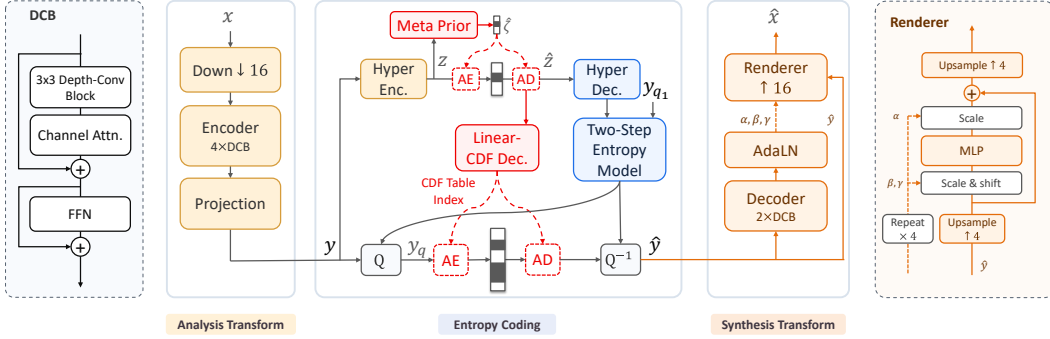
Figure 2: PULSE architecture. It consists of an encoder at 1/16 resolution, a decoupled linear CDF index decoder with a meta prior, a two-step entropy model, and a decoder with an AdaLN-modulated pixel renderer. AE and AD denote arithmetic encoding and decoding, respectively.
