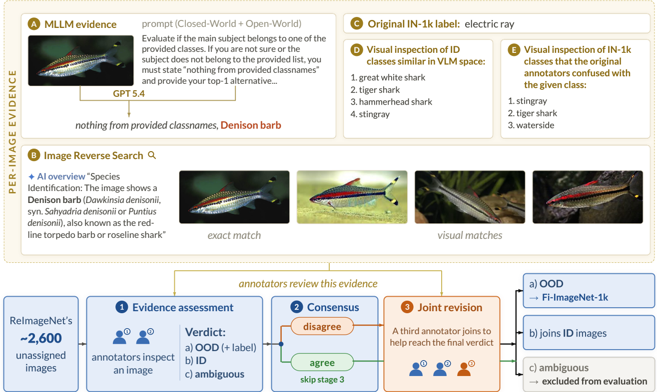
Figure 3. The OOD annotation pipeline. Top: the five sources of per-image evidence an annotator sees, shown here for a Denison barb annotated originally as electric ray . Bottom: the three-stage protocol. 655 images are admitted under consensus and form FI-IMAGENET-1K; images resolved as ID amend in-distribution data, while ambiguous images are excluded from our experiments.
