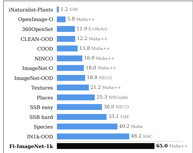
Figure 1. Results for the best-performing EVA02-L model on popular OOD benchmarks that use ImageNet-1k as the in-distribution data, using FPR@95 (↓), in %. Bars show the best (right, in gray) of the 21 post-hoc OOD detectors on a given benchmark. Even for the per-dataset top choice, the FPR@95 on the FI-IMAGENET-1K benchmark is 1.3× higher than on the hardest of the other benchmarks (IN1k-OOD) and 3.8× higher than on recent NINCO.
