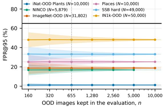
Figure A4. FPR@95 on random subsets and full OOD datasets. Six datasets from Tab. 3, each evaluated on 1000 random n -image draws using EVA02-L-448. For each dataset, the best of the 21 post-hoc detectors is selected on the full dataset and then fixed across all draws; the ID set is also fixed. The plot shows the mean FPR@95 (%), \downarrow over the draws, with bands indicating \pm 2 standard deviations. Dotted lines show the full-dataset values, the solid black line shows FI-IMAGENET-1K as a fixed reference, and the gray vertical line marks n=655 . The mean remains centered on the full-dataset value at every n .
