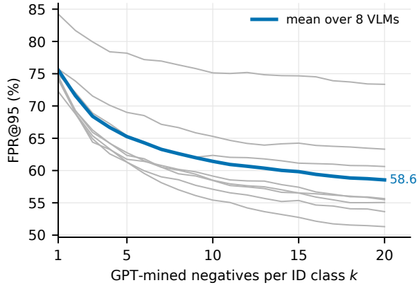
Figure A1. GPT-generated per ID class siblings. FPR@95 (% , ↓) on FI-IMAGENET-1K of NegLabel with GPT-mined per-class siblings as a function of the number k of negatives kept per ID class (gray: the eight VLMs; blue: mean).
