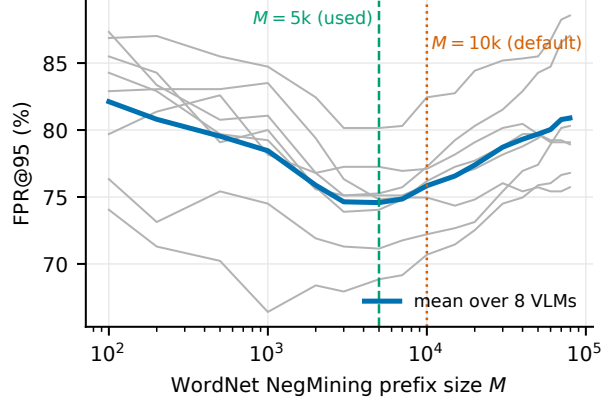
Figure A2. WordNet negative pool size. FPR@95 (% , ↓) on FI-IMAGENET-1K of NegLabel with the NegMined WordNet lexicon as a function of the pool size M (farthest labels first, log scale; gray: the eight VLMs; blue: mean). The default M=10,000 by NegLabel lies past the optimum for every model; Tab. 2 uses M=5000 , the mean of the per-model optima.
