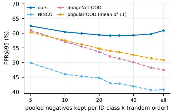
Figure A3. Size of the merged per-ID class negative pool. NegLabel FPR@95 (% , ↓; mean over the eight VLMs) with k negatives kept per ID class from the merged negative pool of all ten GPT-5.4 generations; “all” keeps every candidate (73.6 per ID class on average). More negatives keep helping on popular OOD datasets (dashed) but not on FI-IMAGENET-1K (solid).
