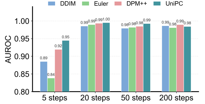
Figure 8: Different ODE solvers with varying inference steps.
