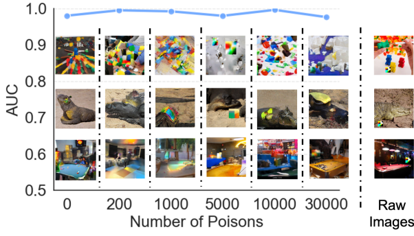
Figure 6: Injecting poisons into the training set.
