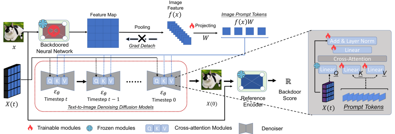
Figure 3: Framework for reconstructing raw pixels from latent representations. Image features are injected into the key/value (K/V) components of the cross-attention module in a pretrained CDDM.
