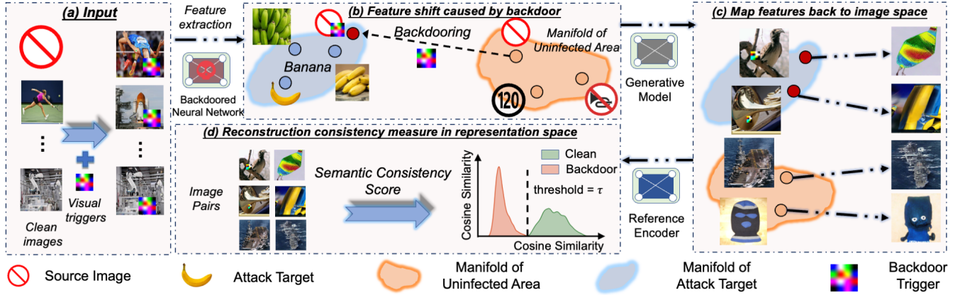
Figure 1: Illustration of the proposed framework for reconstructing backdoor representations back to the image space.
