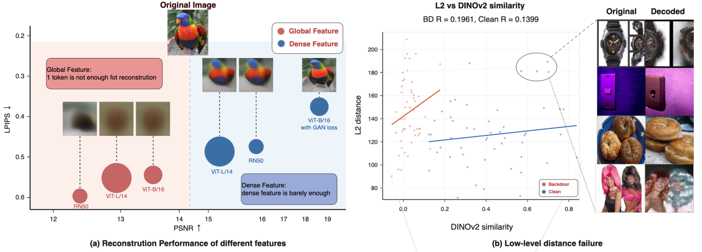
Figure 2: (a) Reconstruction performance across different CLIP encoders [43]. (b) Low-level distance metrics (e.g., L2) fail to reliably assess semantic consistency, as semantically similar images can exhibit high distances.
