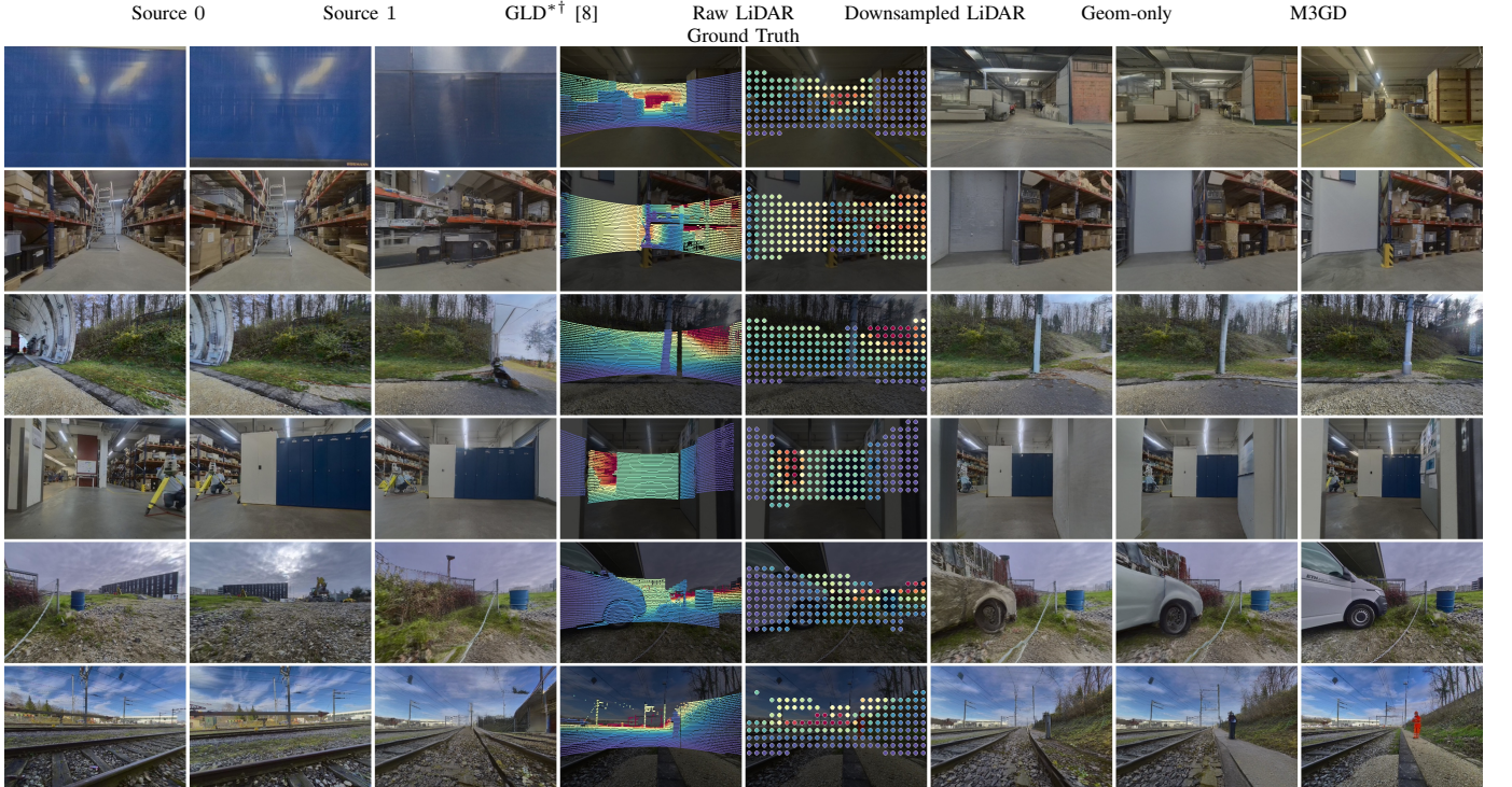
Fig. 7. Qualitative examples highlighting the effect of target-view LiDAR conditioning. Each row shows two source images, the image-only GLD*† baseline, the raw target-view LiDAR projection, our downsampled LiDAR representation, the geometry-only (geom-only) variant, M3GD, and the ground-truth target image. These examples contain large source-target viewpoint changes where RGB-only conditioning is ambiguous and GLD*† often fails to infer the target-facing surface. The LiDAR-conditioned geom-only model recovers the dominant scene layout more accurately, while M3GD further improves appearance fidelity and local details such as boxes, road surfaces, walls, and vehicles by combining LiDAR geometry with Utonia features.
