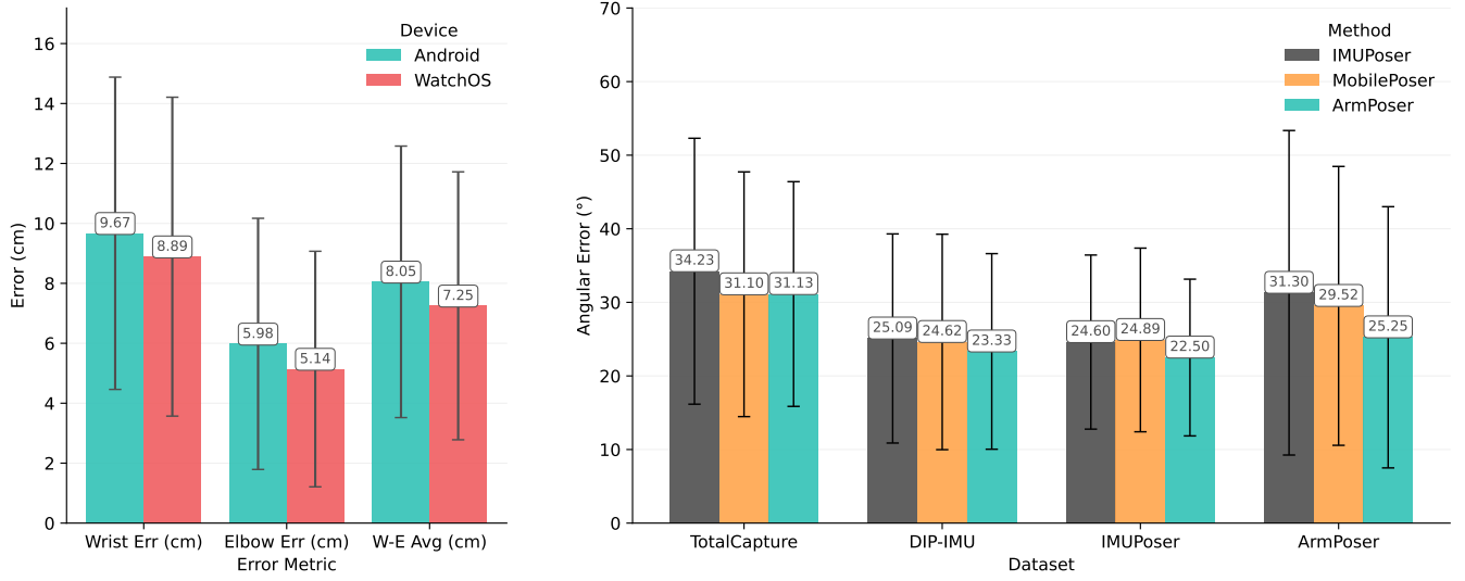
Figure 6: (left) Comparison of positional errors between watchOS and Android smartwatches on the ArmPoser dataset. (right) Comparison of ArmPoser with MobilePoser and IMUPoser in terms of mean angular error across four datasets (TotalCapture, DIP-IMU, IMUPoser, and ArmPoser). Lower values are better; ArmPoser is highlighted in cyan.
