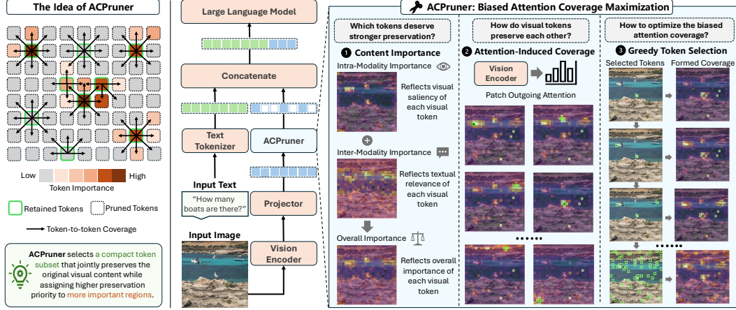
Figure 1: The left part illustrates the core idea of ACPruner. The right part shows how ACPruner is integrated with LVLm inference pipelines and provides a workflow visualization of the method.
