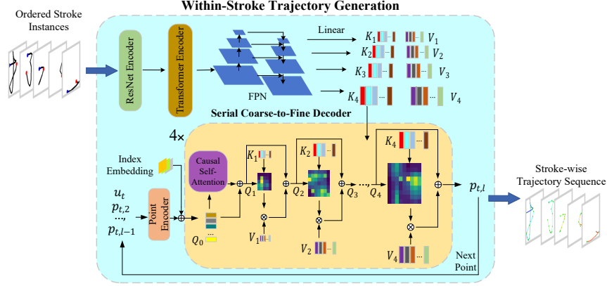
Figure 4: Architecture of the start-point-initialized within-stroke trajectory generation model with serial coarse-to-fine multi-scale decoding.
