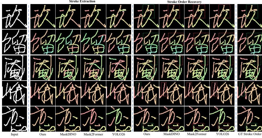
Figure 5: Qualitative comparison of stroke extraction and stroke-order recovery. The left group compares spatial stroke-instance predictions from different models, while the right group compares the corresponding recovered writing orders. Colors in the extraction results distinguish stroke instances only, whereas colors in the order-recovery results are indexed consistently according to writing order. Green and red dashed boxes highlight representative correct and incorrect local stroke-order recovery, respectively.
