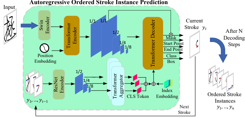
Figure 3: Architecture of autoregressive ordered stroke instance prediction. Previously recovered strokes form the writing history for predicting the current stroke y_t , which is then appended to the history for subsequent decoding.
