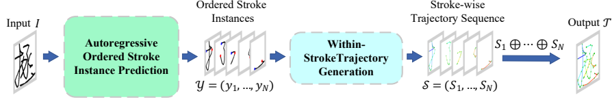
Figure 2: Overview of the proposed two-stage offline-to-online handwriting trajectory recovery framework. The offline image I is first converted into an ordered stroke-instance sequence \mathcal{Y} , followed by stroke-wise trajectory recovery \mathcal{S} and final trajectory concatenation \mathcal{T} .
