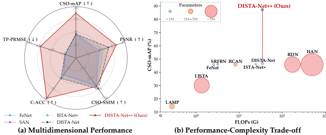
Fig. 8. Comprehensive performance and efficiency comparison on CSIST-100K. (a) Multidimensional Performance: A radar chart benchmarking representative frameworks across five core metrics. Note that the TP-PRMSE (↓) axis is intentionally inverted (the outer edge represents a lower, superior error) to maintain a visually consistent “larger area indicates better overall performance” paradigm. (b) Performance-Complexity Trade-off: Evaluation of CSO-mAP against computational complexity (FLOPs, mapped to a logarithmic x-axis) and network capacity (parameters, represented by bubble area). DISTA-Net++ achieves an optimal balance, dwarfing the performance of heavy architectures at merely a fraction of their computational budget.
