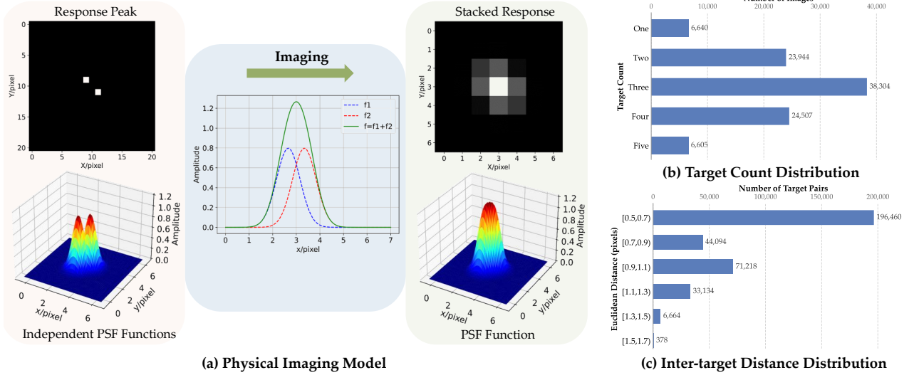
Fig. 3. Overview of the CSIST-100K dataset and the multi-target imaging process. (a) Physical Forward Imaging Model. Illustration of the energy overlap process: (Left) independent sub-pixel point sources and their PSFs; (Middle) a 1D cross-section demonstrating cumulative linear superposition ( f = f_1 + f_2 ); (Right) the final stacked focal-plane response where closely spaced targets merge into a visually indivisible peak. (b) Target Count Distribution. The statistical distribution of images across varying target counts (1 to 5 targets). (c) Inter-target Distance Distribution. The distribution of Euclidean distances (in pixels) between target pairs. The vast majority fall within the extremely close range of [0.5, 0.7] pixels, inducing severe spatial overlap well below the classical resolution limit.
