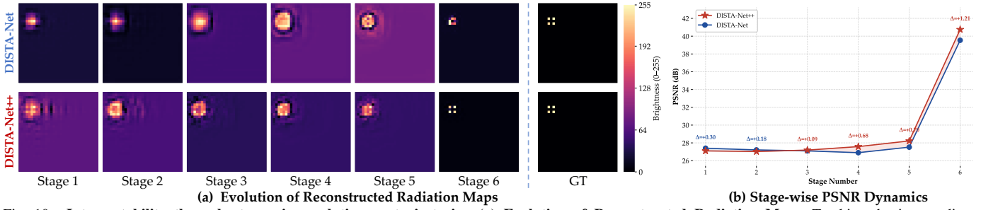
Fig. 10. Interpretability through stage-wise evolutionary trajectories. (a) Evolution of Reconstructed Radiation Maps. Tracking the intermediate representations from Stage 1 to Stage 6 for a highly challenging dense 4-target cluster (Ground Truth shown on the right). While the baseline DISTA-Net merges the cluster into a diffusive blob and ultimately fails to recover the source count, DISTA-Net++ actively suppresses count ambiguity, rapidly converging to four compact, off-grid spatial peaks. (b) Stage-wise PSNR Dynamics. PSNR evolution under identical unfolding depths. The terminal spike reflects the final structural projection from continuous feature manifolds to the discrete radiation map, where DISTA-Net++ decisively outperforms the baseline by expanding the fidelity margin ( \Delta = +1.21 dB).
