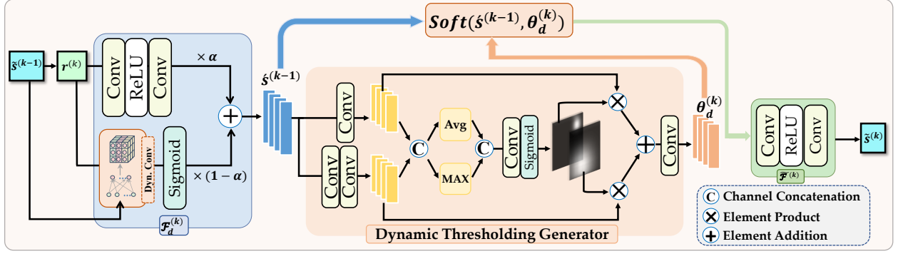
Fig. 6. Architecture of the k -th stage in the dynamic deep unfolding backbone. Each stage contains three main components: a dual-branch dynamic transform module ( \mathcal{F}_d^{(k)} ) for feature extraction, a Dynamic Thresholding Generator (DTG) for feature refinement, and an inverse transform module ( \mathcal{F}^{-1} ) for reconstruction. In the full DISTA-Net++ framework, the DTG is further modulated by a global semantic count prior (omitted in this diagram for visual clarity) to adaptively regulate the thresholds.
