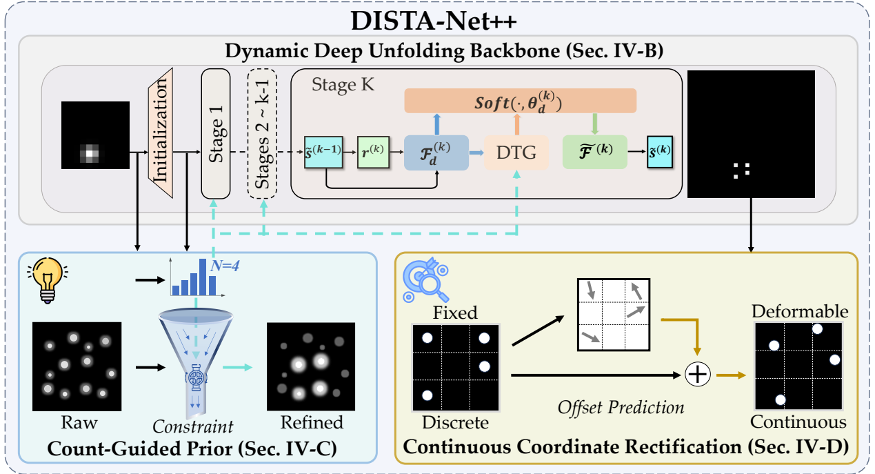
Fig. 5. Overall architecture of the proposed DISTA-Net++. The framework is intrinsically driven by three synergistic components: (a) Dynamic Deep Unfolding Backbone (top) that adaptively extracts features via a Dynamic Transform (DT) module and computes stage-wise soft-thresholds via a Dynamic Thresholding Generator (DTG) to handle sensitive signal variations; (b) Count-Guided Prior module (bottom left) that leverages global target count to semantically modulate features and suppress overlapping ambiguity; and (c) Continuous Coordinate Rectification mechanism (bottom right) that regresses sub-pixel offsets to refine discrete grid estimations into precise continuous spatial localization.
