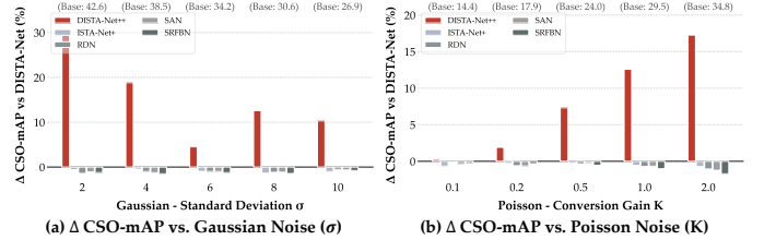
Fig. 13. Robustness against physics-based sensor noise. Relative performance margin ( \Delta CSO-mAP) compared to the DISTA-Net baseline under physically faithful degradation models. (a) \Delta CSO-mAP vs. Gaussian Standard Deviation ( \sigma ). Performance under varying thermal noise standard deviations. (b) \Delta CSO-mAP vs. Poisson Conversion Gain ( K ). Performance under varying photon conversion gains. DISTA-Net++ demonstrates remarkable resilience, maintaining substantial positive margins even as severe physical noise uniformly collapses the baseline performances.
