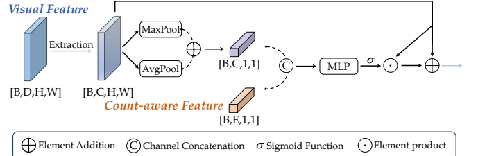
Fig. 7. Detailed architecture of the Count-Aware Modulation (CAM) operation. It effectively integrates the spatial visual features with the semantic count feature to produce channel-wise modulation weights.
