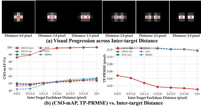
Fig. 11. Robustness across extended inter-target distances. (a) Visual Progression across Inter-target Distances. Evolution from severely mixed (0.5 pixel) to fully isolated (3.0 pixels). (b) (CSO-mAP, TP-PRMSE) vs. Inter-target Distance. While the localization error of grid-based baselines remains clamped to their theoretical quantization floor regardless of inter-target distance, DISTA-Net++ utilizes continuous regression to drive sub-pixel error toward zero as spatial overlap relaxes.
