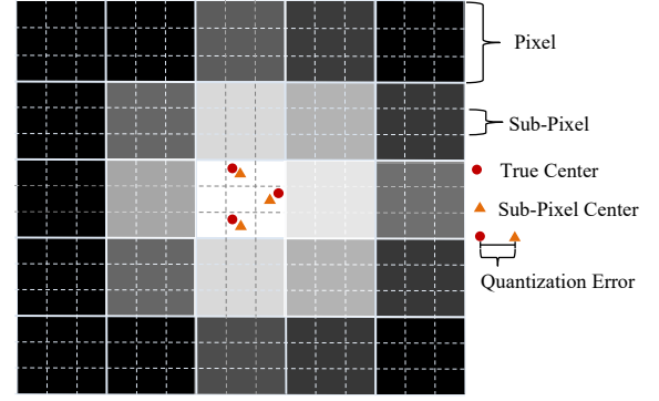
Fig. 4. Division of each pixel into an n \times n grid of sub-pixels, representing potential target positions.
