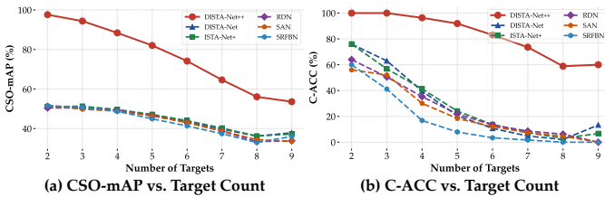
Fig. 12. Robustness under extended target count. Evaluation as cluster density scales across the expanded range (plotted from 2 to 9 targets). (a) CSO-mAP vs. Target Count. The trajectory of overall sub-pixel detection performance. (b) C-ACC vs. Target Count. The trajectory of semantic count estimation. Even when trained on datasets containing these extremely dense configurations, baselines suffer systemic semantic collapse, whereas DISTA-Net++ sustains a commanding accuracy lead.
