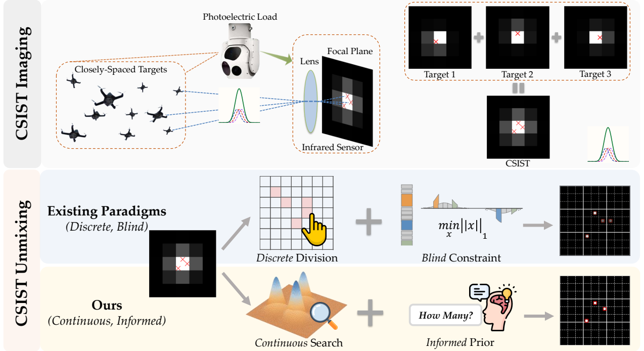
Fig. 2. Conceptual illustration of imaging and unmixing processes for closely-spaced infrared small targets (CSIST). CSIST unmixing aims to disentangle and accurately estimate the count, positions, and intensities of overlapping targets.
