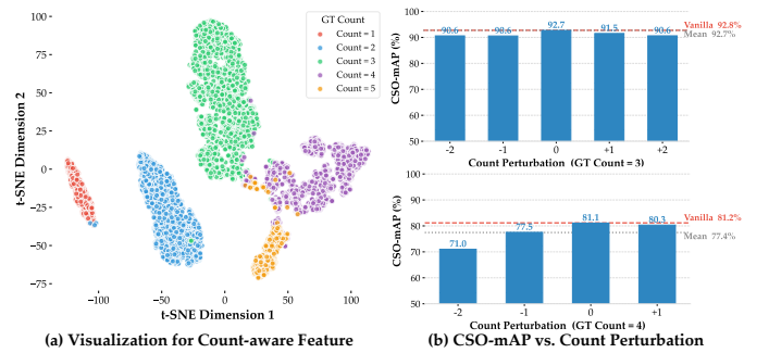
Fig. 14. Mechanism validation of the Count-Guided Prior. (a) Visualization for Count-aware Feature. A t-SNE projection of the count embedding \mathbf{c} , demonstrating distinct semantic clustering aligned with the ground-truth target count. (b) CSO-mAP vs. Count Perturbation. Performance under count perturbations. Injecting the exact ground-truth embedding (0 perturbation) establishes the theoretical upper bound, which the default predictive model (Vanilla) closely matches. Injecting erroneous embeddings ( \pm 1, \pm 2 ) demonstrates graceful degradation, proving the framework’s robustness against counting errors.
