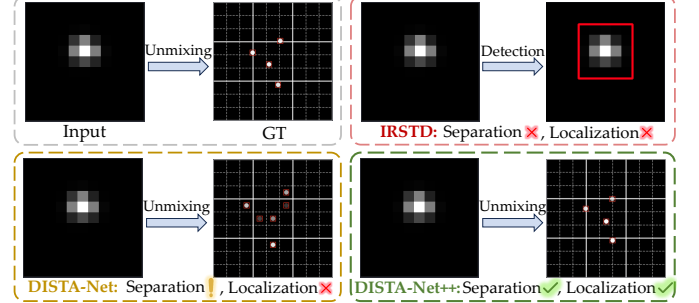
Fig. 1. Evolution of processing paradigms for closely-spaced infrared small targets (CSIST). Top right: Infrared Small Target Detection (IRSTD) acts only as a coarse detector, reporting a single bounding box for overlapped targets. Bottom left: Existing unmixing models (e.g., DISTA-Net) succeed in separating the overlapped signals, yet in a blind, discrete manner, thus suffering from count ambiguity and grid quantization error. Bottom right: The proposed DISTA-Net++ establishes an informed, continuous formulation, achieving faithful recovery of target count, sub-pixel positions, and intensities aligned with the Ground Truth (GT). Unmixing results are shown cropped and enlarged around the target region for clarity.
