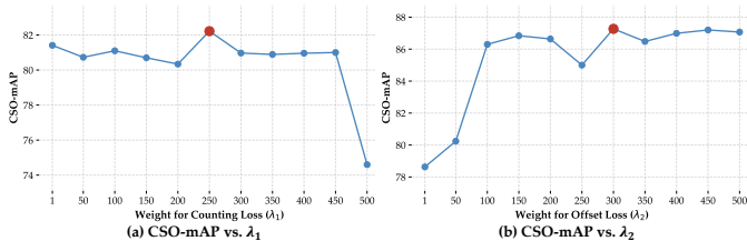
Fig. 15. Ablation study on loss weight sensitivity. (a) CSO-mAP vs. \lambda_1 . The effect of the counting loss weight on sub-pixel detection performance. (b) CSO-mAP vs. \lambda_2 . The effect of the offset loss weight. The red dots indicate the optimal settings adopted in our final model ( \lambda_1 = 250 and \lambda_2 = 300 ). The broad plateaus across both metrics demonstrate that the framework is highly robust and avoids delicate hyperparameter tuning.
