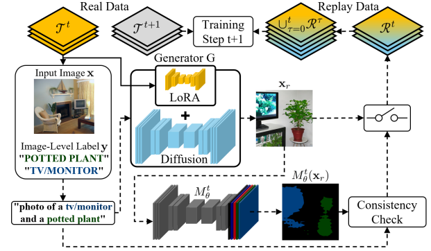
Fig. 1. Overview of the DR.WILSS replay strategy: at each training step the segmentation network is trained with a combination of real data and replay samples from the generative module. During training, representative captions are acquired to be used in conjunction with a LoRA module trained on the step data to control the generative model in the next step. A post-generation consistency check ensures that all prompted classes are present.
