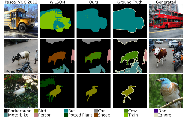
Fig. 3. Qualitative results for the overlapped 15-5 scenario.
