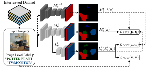
Fig. 2. At step t > 0 , the model is trained on new data and replay data of previous classes. The localizer and previous model provide pseudolabels.
