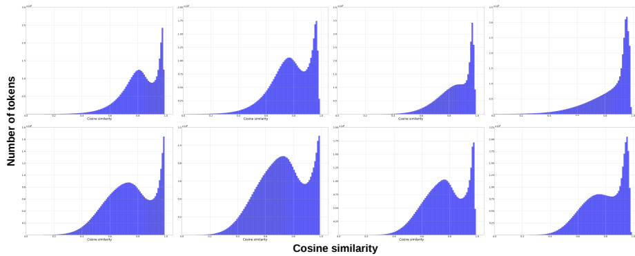
Fig. 3: Distributions of cosine similarities between adjacent tokens in Seg across backbone sizes. From left to right: T, S, B and L backbone sizes. From top to bottom: distributions computed at 1st and 2nd layers. The decoder is a Mask Transformer. The distributions are computed over the training set of ADE20K.
