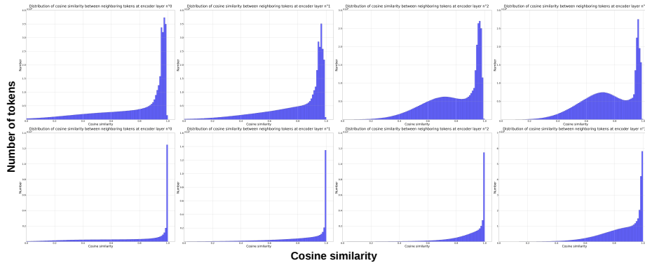
Fig. 6: Distributions of cosine similarities between adjacent tokens in EoMT. From top to bottom: AugReg and DINOv2 pretraining weights. From left to right: distributions computed at 1st, 2nd, 3rd and 4th layers. The distributions are computed over the training set of ADE20K.
