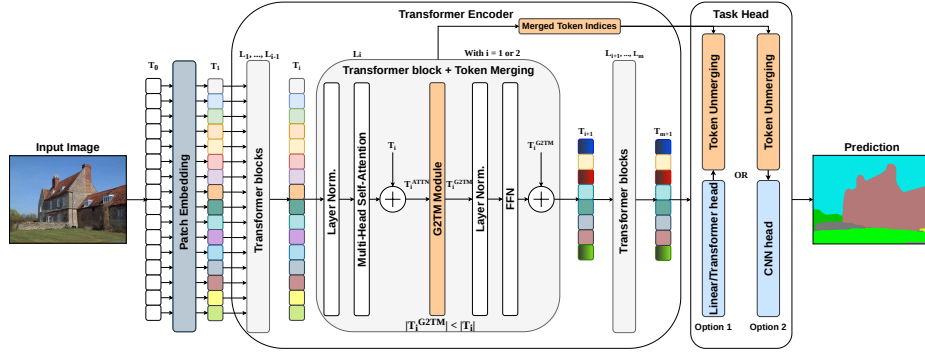
Fig. 1: Integration of the G2TM module within the i^{th} Transformer block of a ViT-based architecture. The module is inserted following the attention layer and the residual connection of one of the shallow Transformer blocks (typically, i = 1 or 2 ).
