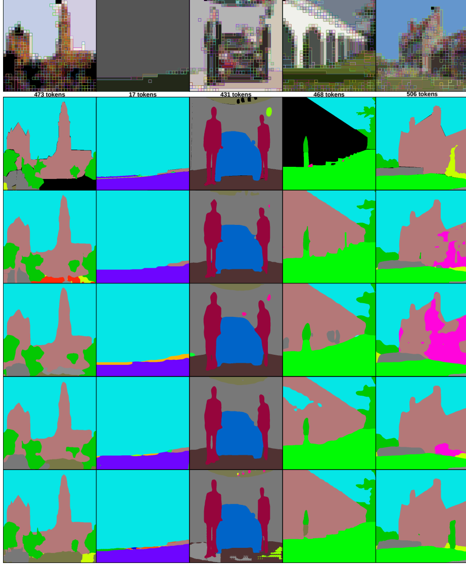
Fig. 5: Visualization of fused tokens and segmentation maps. From top to bottom: fused token layout of G2TM applied to Seg with Mask Transformer decoder; ground truth segmentation maps; segmentation maps predicted by the latter Seg model; SETR-PUP; SETR-MLA; and EoMT. For all models, the backbone is a ViT-L and G2TM is applied at the second layer.
