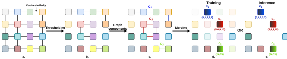
Fig. 2: Illustration of G2TM merging strategy. Tokens are arranged on a 2D grid. Their position in the grid corresponds to those of the patches in the original image. The final merging operation (last step) differs between training (left) and inference (right): during training, merged tokens are masked for self-attention (depicted as transparent), whereas during inference, they are entirely removed.
