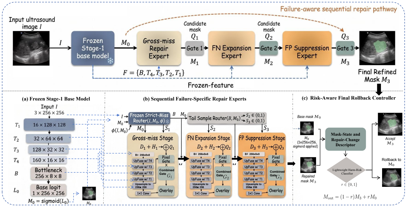
Figure 2: Overview of FAPR. The frozen base model provides the initial mask M_0 and a shared multi-scale feature pyramid. Three failure-specific experts sequentially propose complete candidate masks Q_k , and the corresponding gates selectively overlay each candidate on the latest state to produce M_1 , M_2 , and M_3 . A lightweight risk-aware controller finally accepts M_3 or rolls the prediction back to M_0 .
