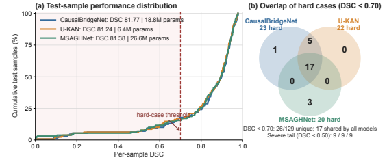
Figure 1: Persistent hard-case tails on BUSI. (a) Per-sample DSC distributions with model averages and parameter counts. (b) Among cases below 0.70 DSC, 17 are shared by CausalBridgeNet, U-KAN, and MSAGHNet.
