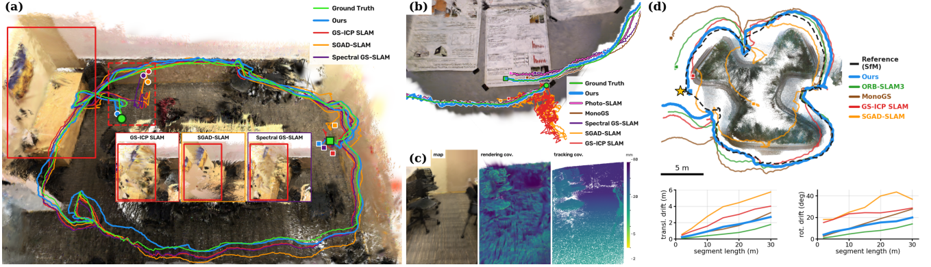
Fig. 1: Our method tracks robustly in various challenging conditions, such as indoor loops in (a) compared to other ICP methods, and in structure-less scenes rivaling MonoGS and Photo-SLAM in (b), and in outdoor scenes (d) shows the lowest drift among evaluated 3DGS-based methods. We do this by maintaining two covariances per Gaussian: one for rendering, and one for tracking, as shown in (c), colored by the size of the respective covariances.
