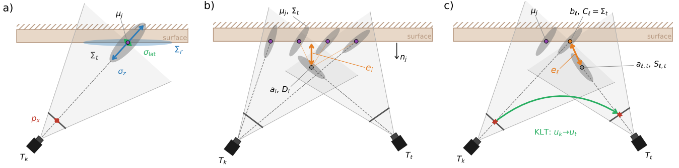
Fig. 2: System Overview. (a) We define each Gaussian to consist of a photometrically optimized covariance \Sigma_r and a sensor measurement uncertainty covariance \Sigma_t . (b) The depth residuals are defined by the standard G-ICP cost with the source covariance D_i defined as the observation’s uncertainty. (c) The image residuals are defined as KLT corners anchored to nearby Gaussians, with uncertainty defined by the anchor’s covariance.
