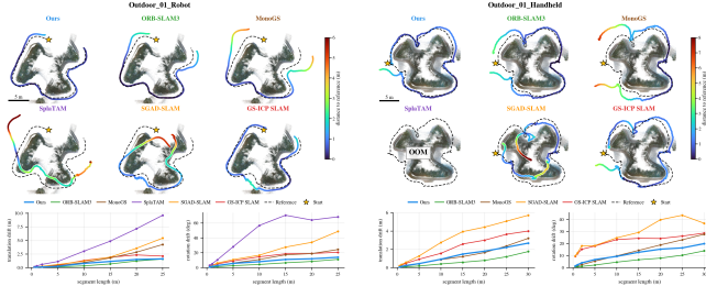
Fig. 3: Performance on outdoor scenes. Ours has the lowest drift of all evaluated 3DGS SLAM methods in both the wheeled-platform (left) and handheld settings (right) on up to 70m+ length trajectories.
