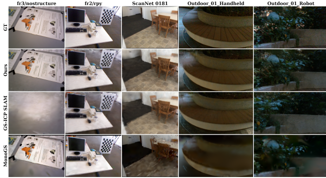
Fig. 4: Qualitative render quality of our method compared to some baselines. We render scenes from TUM RGB-D, ScanNet, and from our custom sequences.
