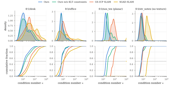
Fig. 5: Comparison of condition number across ICP methods. Ours reduces the condition number in general, indicating that the optimization is more well-constrained.
