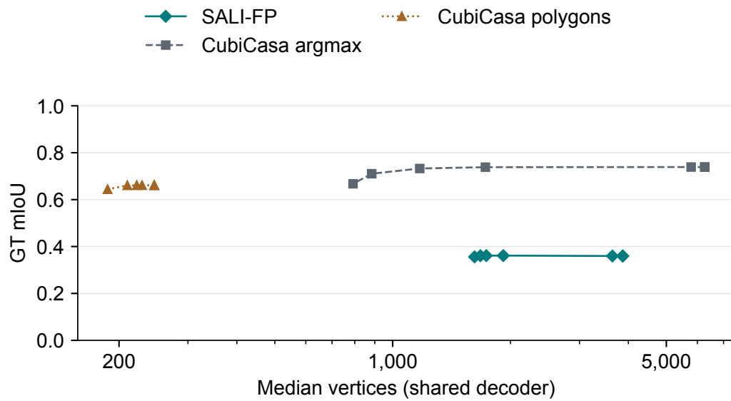
Fig. C.3: GT accuracy versus shared-decoder control-point cost at the seven fixed simplification tolerances in Table C.13. Every setting is applied to all test plans; no per-plan selection uses GT. Markers denote the frozen tolerance settings.
