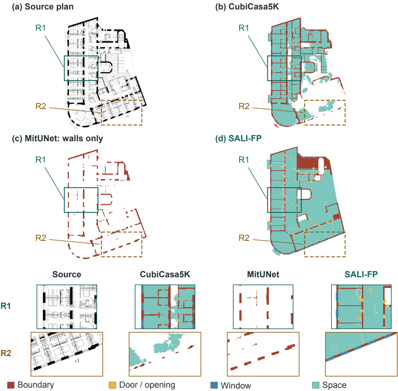
Fig. F.23. archp10k_000872: repeated hotel entrances and a diagonal lower wing.
