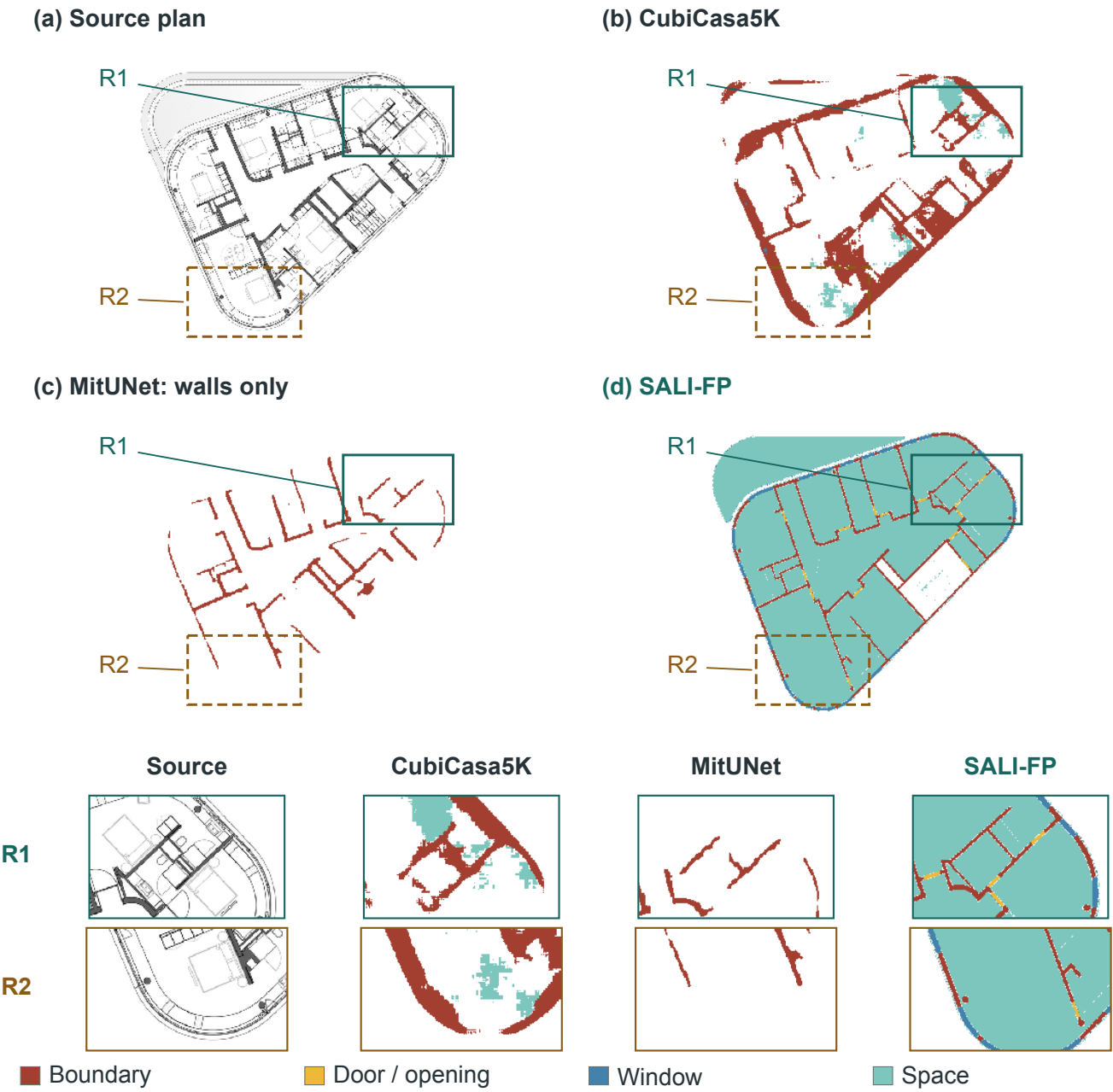
Fig. F.10. archp10k_000896: curved hotel perimeter and oblique room wings.
