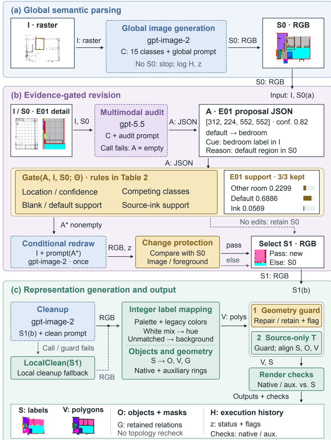
Fig. 2: SALI-FP architecture and evidence flow: (a) global semantic parsing; (b) evidence-gated revision and protected candidate selection; (c) representation generation and a connected output package. Rounded containers group operations; rectangular frames contain data and recorded evidence. Arrows identify data or selection conditions. The frozen CubiCasa5K test 0002 example supplies the images and E01 record; three accepted proposals illustrate the recorded evidence-gated execution. G retains generated relations. The local geometric extension is evaluated as a subsequent representation stage.
