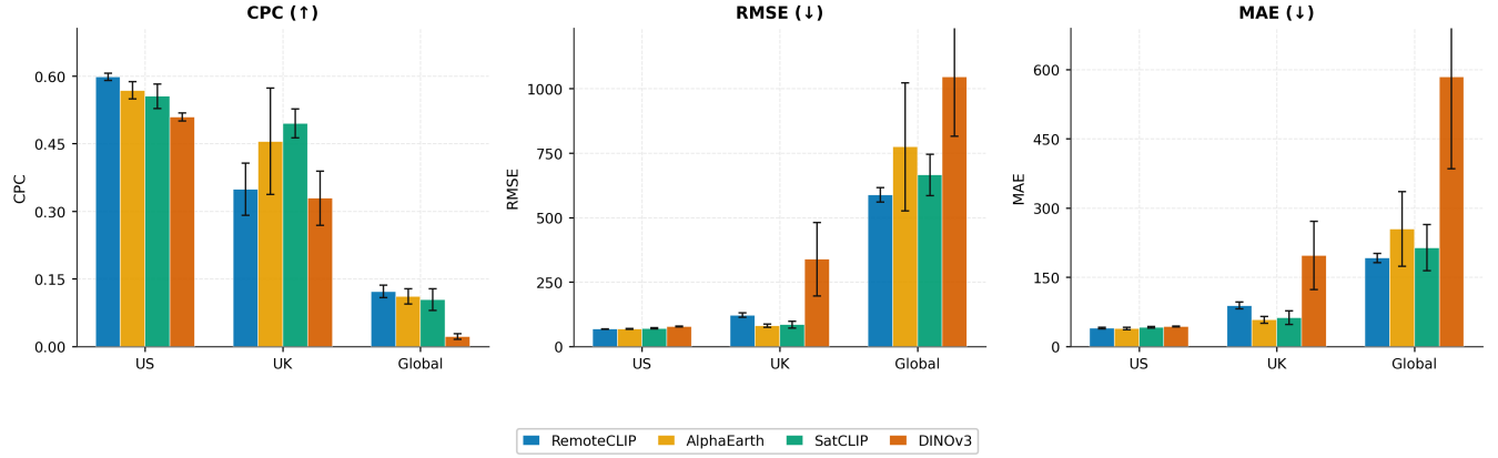
Figure 2: Mean CPC, RMSE, and MAE per region across all \eta levels (mean \pm std, 5 seeds), consistent with Table 3. RemoteCLIP leads in-distribution (US); SatCLIP and AlphaEarth dominate zero-shot UK transfer; all encoders converge on Global cities. DINOV3 collapses to near-zero performance globally (CPC = 0.022).
