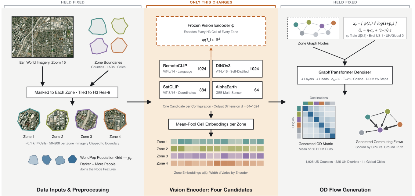
Figure 1: GLODGen pipeline. Satellite imagery and population data are preprocessed via H3 hexagonal tiling (resolution 9, \sim 0.1 \text{ km}^2 per cell) with per-tile mean pooling. A spatial vision encoder extracts zone-level embeddings conditioning the WeDAN GraphTransformer diffusion model, which generates the OD flow matrix via DDIM sampling.
