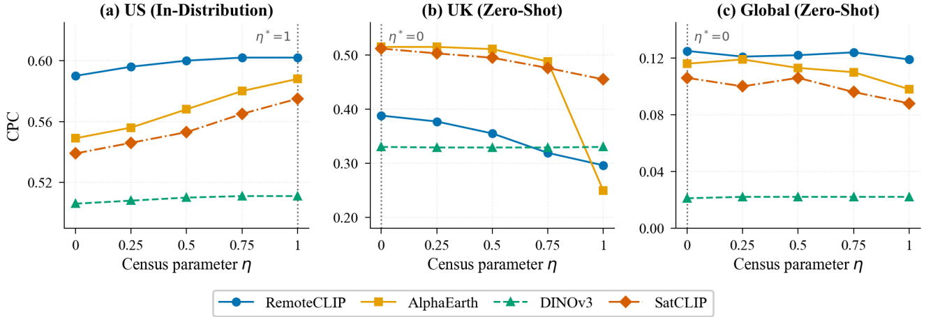
Figure 3: CPC as a function of census noise parameter \eta across all four encoders and three evaluation benchmarks (mean over 5 seeds). The dashed vertical line marks the primary evaluation point for each dataset ( \eta=1 for US; \eta=0 for UK and Global). US performance increases monotonically with census availability, whereas UK and Global performance degrades as \eta \rightarrow 1 due to the introduction of out-of-distribution zero-valued census vectors.
