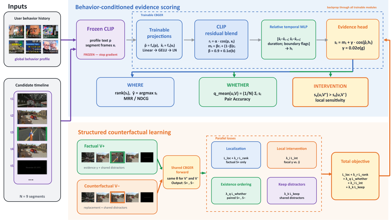
Figure 3. Behavior-conditioned evidence scoring and structured counterfactual learning. Frozen CLIP features are processed by lightweight projections, a CLIP residual branch, and a relative-temporal MLP to produce segment evidence logits. Their ranking answers Where , while parameter-free mean pooling answers Whether . Factual V^+ and matched counterfactual V^- share parameters and are jointly supervised by localization, existence-ordering, local-intervention, and distractor-invariance losses. Gradients update only the lightweight CBGER scorer; CLIP remains frozen.
