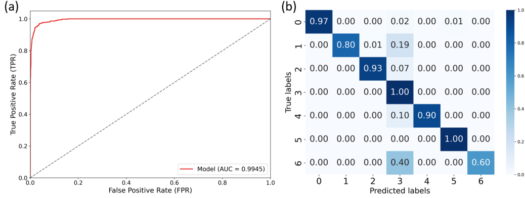
Figure 7: (a) ROC curves with AUC values and (b) the confusion matrix of CUA-Net on the external test cohort. 0-6 denotes: normal uterus, septate uterus, arcuate uterus, unicornuate uterus, uterus didelphys, T-shaped uterus, bicornuate uterus, respectively.
