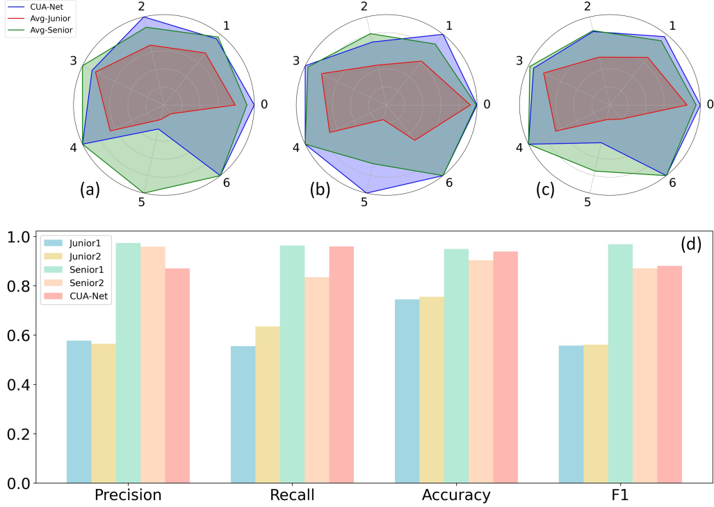
Figure 5: Performance comparison between CUA-Net and junior/senior sonographers. Radar charts illustrate (a) precision, (b) recall, and (c) F1-score across different categories (0-6: normal uterus, septate uterus, arcuate uterus, uterus didelphys, unicornuate uterus, T-shaped uterus and bicornuate uterus) for CUA-Net (blue), average juniors (red), and average seniors (green), respectively. (d) Bar chart presents the overall precision, recall, accuracy, and F1-score of juniors (Junior1/2), seniors (Senior1/2), and CUA-Net.
