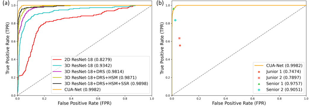
Figure 3: ROC curves with AUC values for (a) different methods and (b) junior and senior sonographers. The AUC values for sonographers are approximated by connecting several points, i.e., (0,0), (FPR, TPR), and (1,1), following [29].
