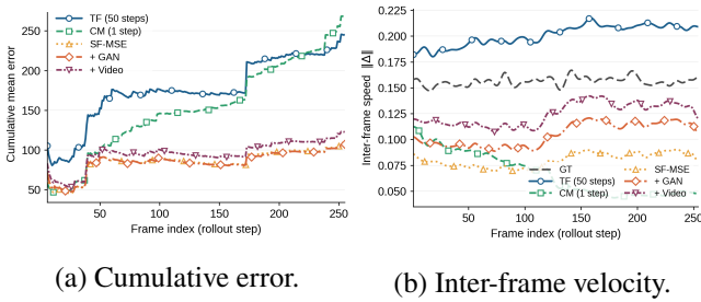
Figure 4: Exposure bias across variants. TF models drift over the rollout (a); SF variants curb this drift, and distribution-matching objectives restore GT-level velocity (b).
