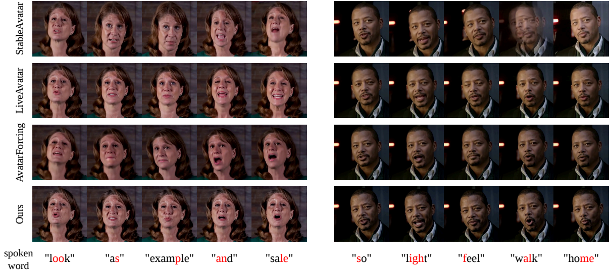
Figure 3: Qualitative comparison with Wan-based end-to-end methods. For each result we show five frames with the spoken word beneath; the phoneme being articulated is highlighted in red (e.g. the “oo” in “look”), so that lip shape can be checked against the sound at each frame. Our method produces the tightest audio–lip alignment and the sharpest facial detail.
