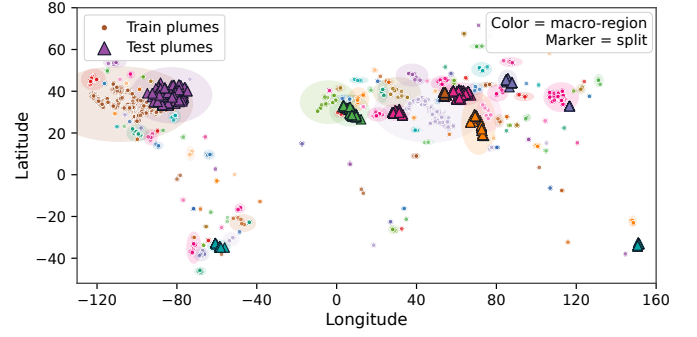
Fig. 7. Geo-cluster split for spatial robustness evaluation. Plume reports are grouped into tile-scale clusters and 275 km macro-regions, and each macro-region is assigned entirely to training or testing.
