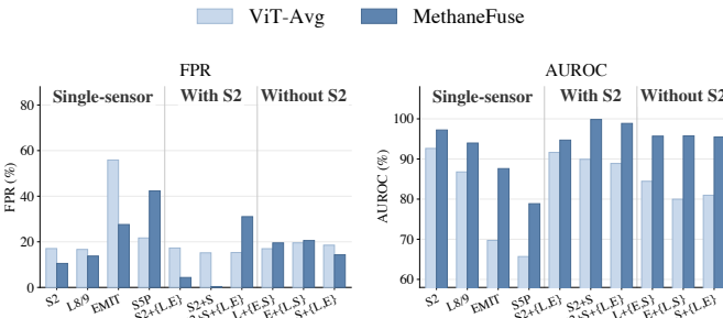
Fig. 6. FPR and AUROC for the sensor-set transfer groups in Fig. 5. Rows compare the per-sensor ViT average-fusion baseline with MethaneFuse .
