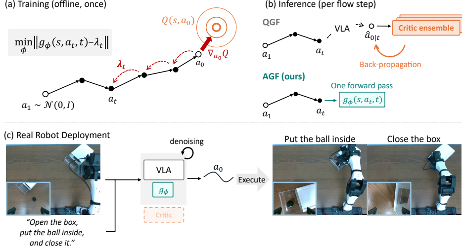
Figure 1: Overview of AGF. (a) Training: the terminal critic gradient is carried back through the frozen flow and regressed into g_{\phi} . (b) Inference: QGF back-propagates a critic ensemble per step; AGF runs one forward pass of g_{\phi} . (c) Deployment on a real robot, with no critic ensemble on board.
