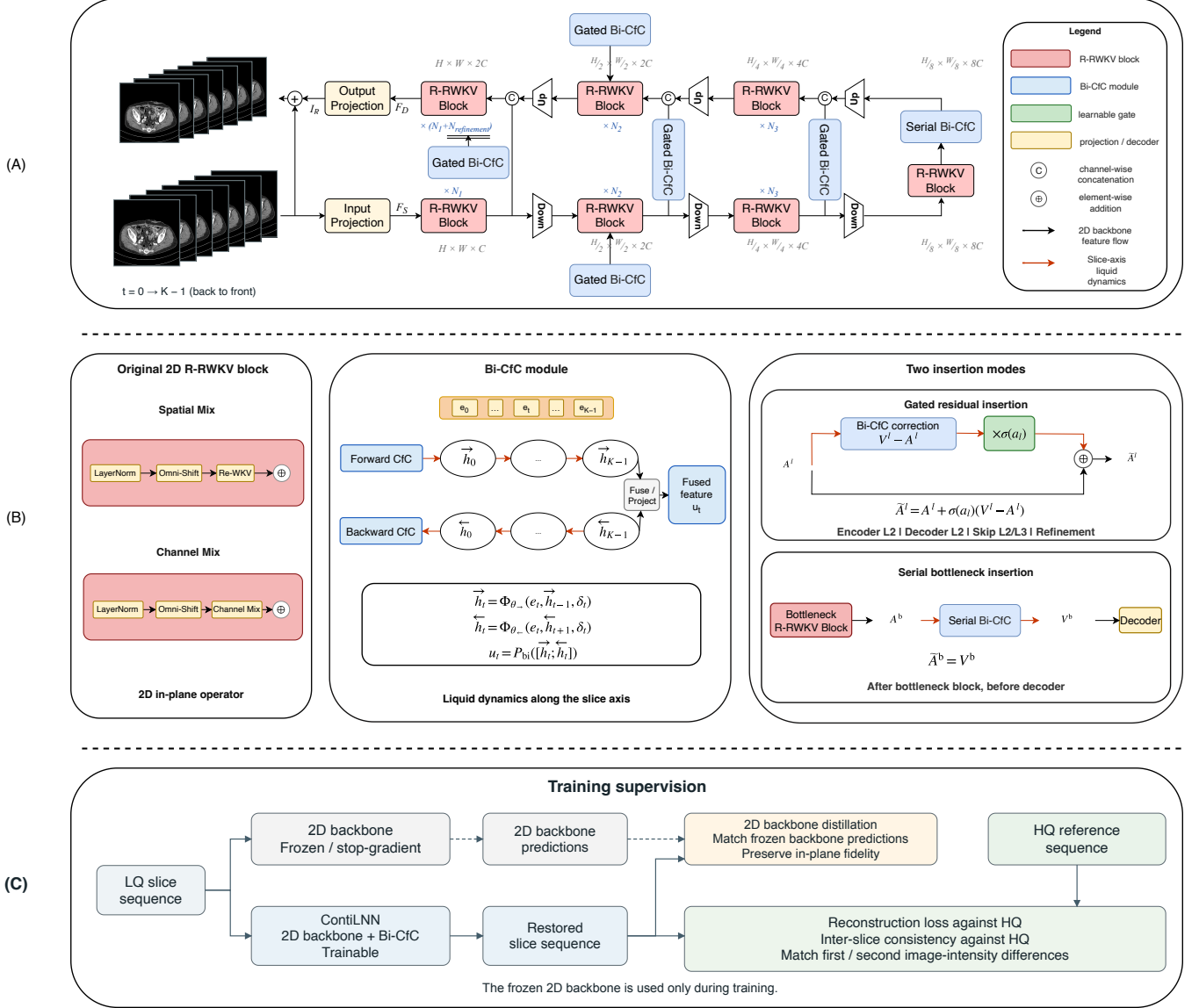
Figure 2: ContilLNN architecture based on Restore-RWKV (Yang et al., 2026a). (A) Bi-CfC modules augment selected feature pathways; the paired CT sequences show the same seven observed positions, ordered back to front. (B) Backbone blocks, the bidirectional liquid operator, and gated residual or serial insertion. Reverse traversal preserves feature–interval pairing (Eq. 10). (C) Training supervision. High-quality references supervise reconstruction and first- and second-order inter-slice intensity differences. A frozen 2D backbone supplies single-slice predictions for distillation during training; the ContilLNN backbone and Bi-CfC modules remain trainable.
