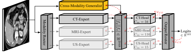
Fig. 1: Schematic representation of GS-MoE with the Expert Classifier. Showing an exemplary forward (black) and backward (red) pass for a CT input. Training is performed in stages, with each part trained on its relevant subset of data.
