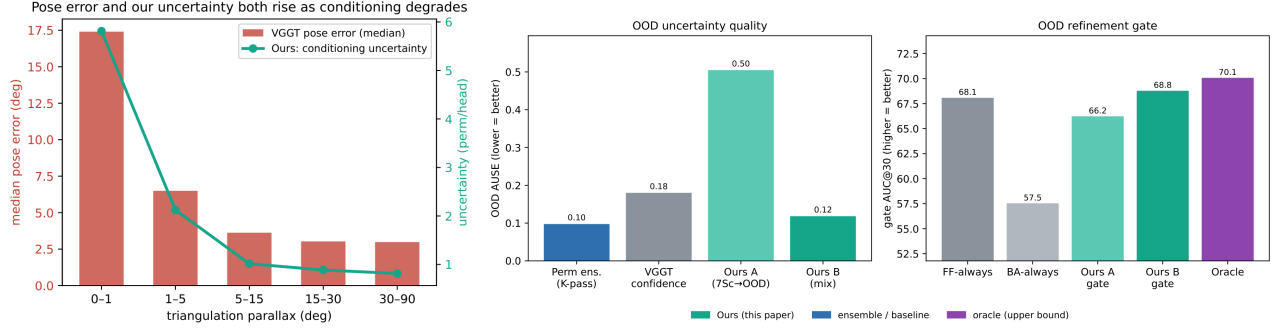
Figure 3. Conditioning explains failures and decisions. Left: pose error and orbit-variance uncertainty rise as parallax degrades, while native confidence remains weakly informative. Right: on the OOD outdoor extreme-view benchmark, the orbit teacher and one-pass head outperform native confidence as reliability signals, and the gate avoids the damage caused by applying BA uniformly.
