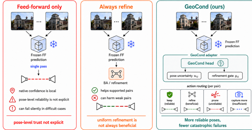
Figure 1. GeoCond as a pose-level reliability adapter. Feed-forward-only prediction provides no explicit pose-level trust signal and can fail silently in difficult cases, while uniformly applying bundle adjustment may help supported pairs but harm weak ones. GeoCond augments a frozen feed-forward backbone with conditioning features to predict pose uncertainty and a refinement gate, selectively keeping, refining, pruning, or requesting additional views for each relative pose.
