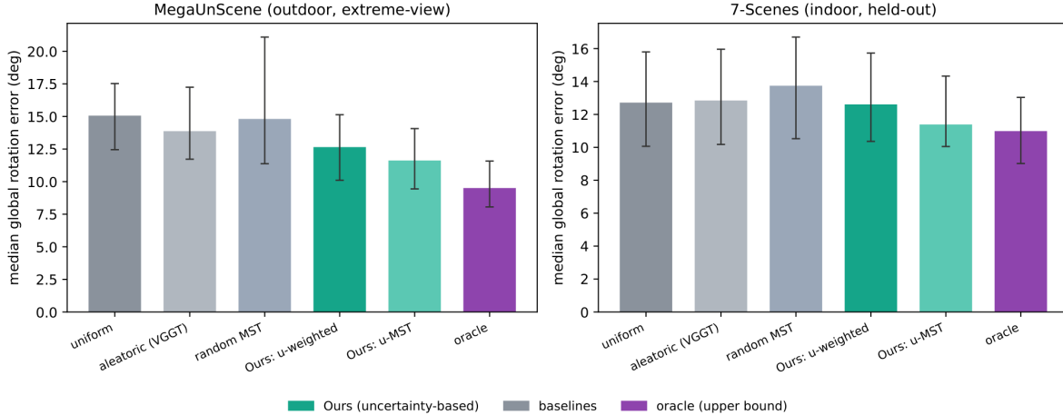
Figure 5. Downstream pose-graph fusion from independent pairwise VGGT estimates ( N = 6, 80 view sets). Bars show median global rotation error with bootstrap 95% CIs. Uncertainty-weighted and uncertainty-selected edges improve rotation averaging on MegaUnScene; gains are smaller indoors.
