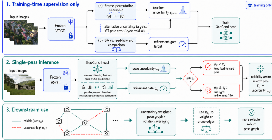
Figure 2. Overview of GeoCond. In the default VGGT setting, training uses a frozen backbone to generate an uncertainty teacher from frame-permutation orbit variance and a refinement target from BA-vs-feed-forward comparison. More generally, the reliability teacher can also come from target-domain pose errors or cycle residuals from unlabeled pose graphs. At inference, the backbone runs once and a lightweight GeoCond head predicts pose uncertainty u_{ij} and a refinement gate g_{ij} from conditioning features derived from the backbone’s own predictions. The predicted uncertainty can also weight or prune edges in a downstream pose graph.
