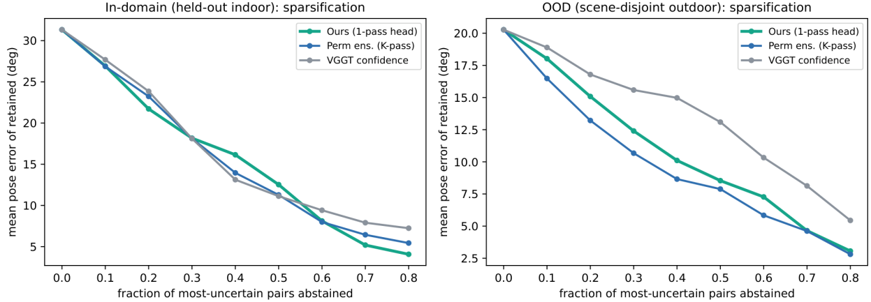
Figure 4. Sparsification curves: mean pose error of retained pairs after abstaining from the most uncertain predictions. The one-pass head and the orbit teacher track pose error substantially better than native confidence.
