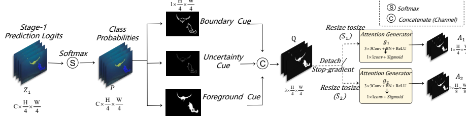
Fig. 4. Prediction-Cued Dual-Stage Decoder.
