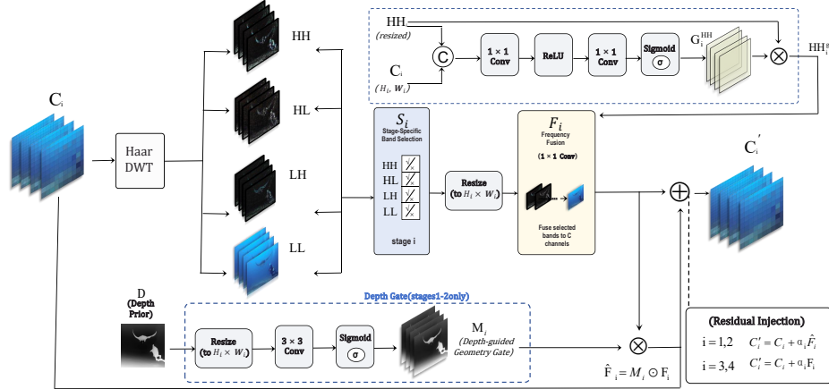
Fig. 3. Stage-Specific Wavelet Representation with Geometry-Guided Gating
