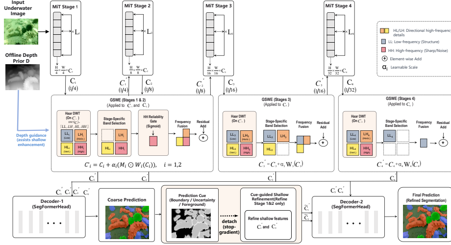
Fig. 2. Overall architecture of GeoCueFormer.
