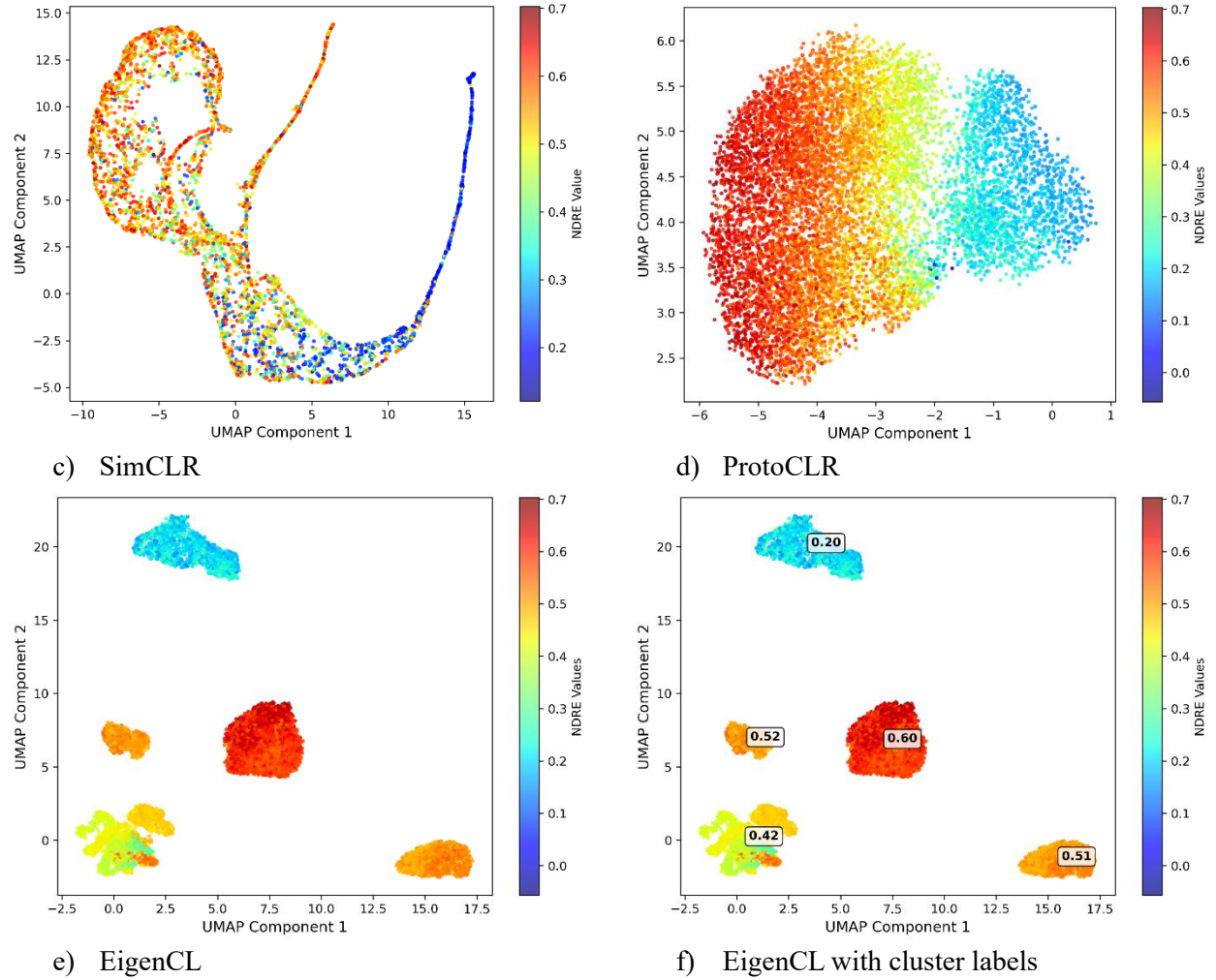
Figure 7: Embedding and stress clustering comparison on the Iowa dataset.
