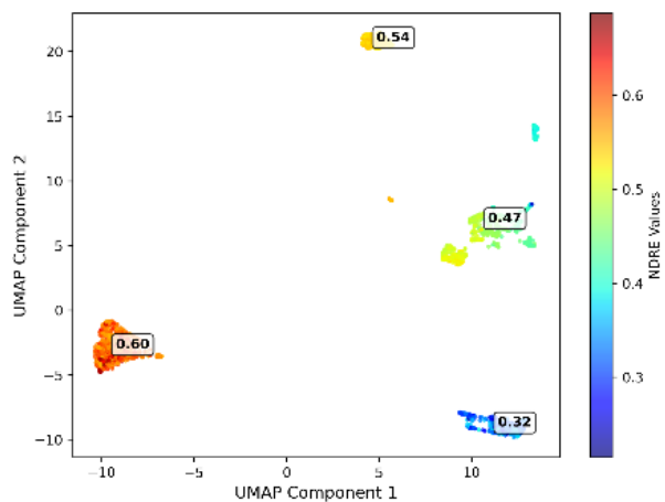
f) EigenCL with cluster labels
