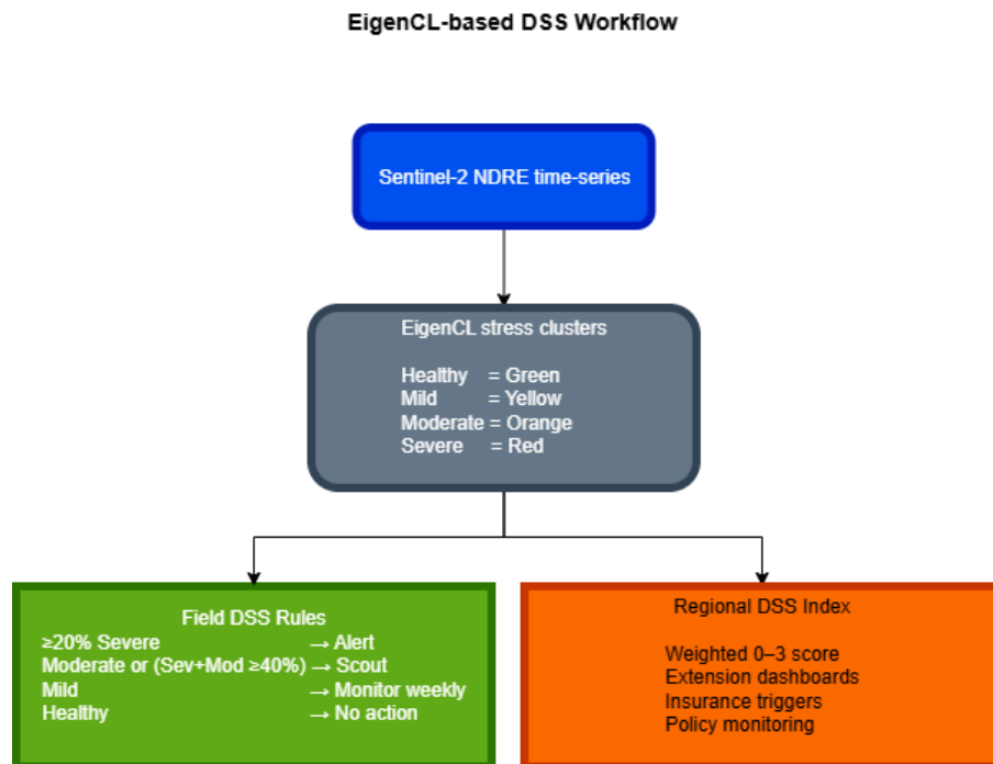
Figure 10: Workflow for integrating EigenCL into a Decision Support System (DSS). Sentinel-2 NDRE time-series are processed by the EigenCL model to produce four stress clusters (Healthy, Mild, Moderate, Severe). Outputs can then be used at the field level to trigger scouting or irrigation actions through cluster-based rules, and at the regional level to build stress indices for extension dashboards, crop insurance, and policy monitoring.
