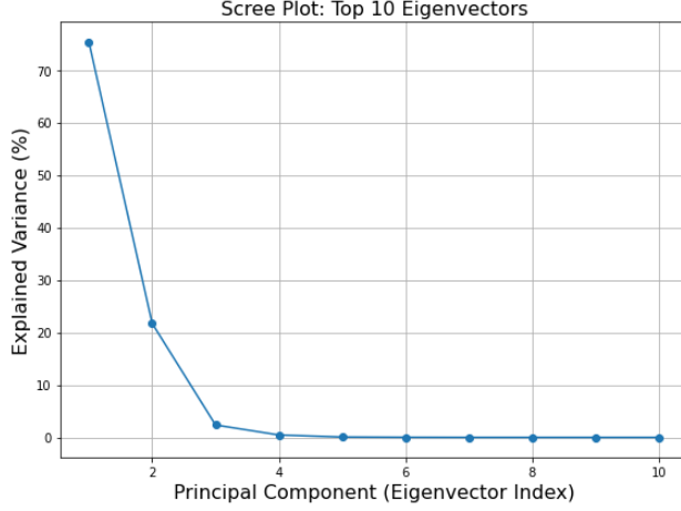
Figure 4. The plot shows how much variance is explained by each eigenvector. The first eigenvector alone captures a dominant share (~76%) of the total variance, justifying its use as the principal signal for guiding contrastive learning.
