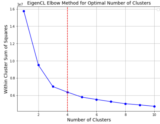
Figure 6: Elbow method to determine the optimal number of clusters from EigenCL embeddings.
