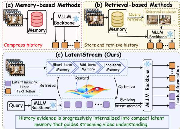
Figure 1: Motivation of our LatentStream : paradigm comparison of memory-based and retrieval-based methods with our retrieve-and-internalize method LatentStream .
