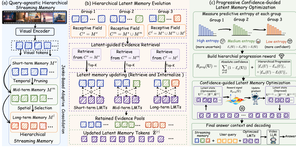
Figure 2: The overview of LatentStream . (a) Query-agnostic hierarchical streaming memory (HSM) organizes incoming visual tokens into short-, mid-, and long-term memories via Jenks-based adaptive consolidation. (b) Hierarchical latent memory evolution (HME) retrieves and internalizes historical evidence into compact latent memory via progressively expanding memory receptive fields. (c) Progressive confidence-guided latent memory optimization (PMO) refines the latent memory tokens with a hierarchical progression reward for streaming reasoning.
