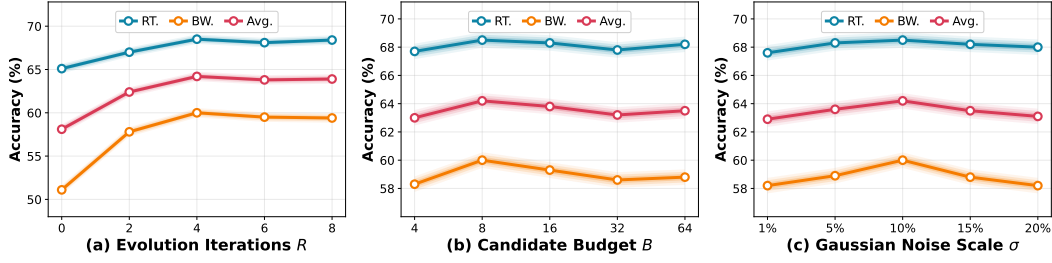
Figure 3: Hyperparameter analysis on OVO-Bench [30] . (a) Effect of the number of evolution iterations R . (b) Effect of the candidate budget B . (c) Effect of Gaussian noise scale \sigma . “RT” / “BW” denote Real-Time Visual Perception and Backward Tracing; “Avg.” is the mean of RT and BW.
