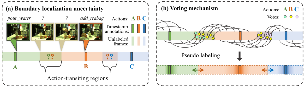
Fig. 1. (a) Due to the inherent feature ambiguity in action-transiting regions, existing works suffer from significant uncertainty in boundary localization, resulting in inaccurate frame-wise pseudo-label generation and cascaded performance deterioration. (b) Our network propagates and aggregates key action representations as votes into the action-transiting regions, thereby refining boundary localization and improving segmentation performance in both the training and testing phases.
