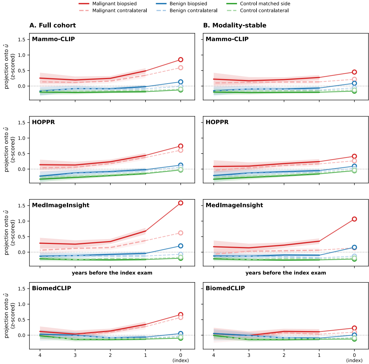
Figure 5: Group mean projection of biopsied and contralateral breast embeddings onto the cancer direction \hat{u} . (A) Full cohort. (B) Modality-stable patients only. Each group is plotted as a biopsied side (dark, solid) and contralateral side (light, dashed) pair: malignant (red), benign (blue), and control (green). In both malignant and biopsy-negative arms the biopsied side separates above the contralateral side toward the index, and the split persists under the restriction of modality stability (B). Conversely, the control group breasts overlap in trajectory, yielding a null result. The index exam is shown as open circles on a dashed segment.
