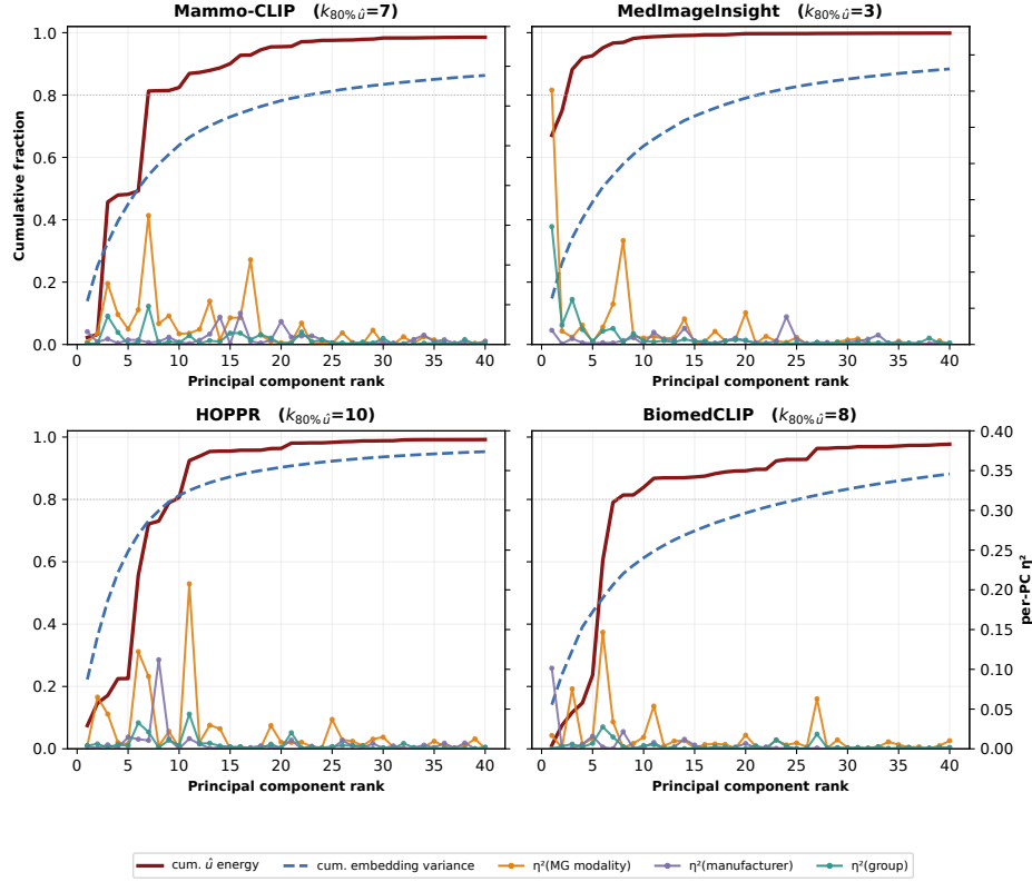
Figure S1: PCA probe (breast-level, L2-normalized embeddings + longitudinal ComBat). For each model, we plot the cumulative \hat{u} energy (red) and cumulative embedding variance (blue dashed) by PC rank (left axis) and per-PC \eta^2 for modality, manufacturer, and the biological group label (right axis). \hat{u} is concentrated in high-variance PCs for Mammo-CLIP, MedImageInsight, and BiomedCLIP but diffuse for HOPPR (80% of \hat{u} energy by PC 7/3/8 vs. PC 10, respectively).
