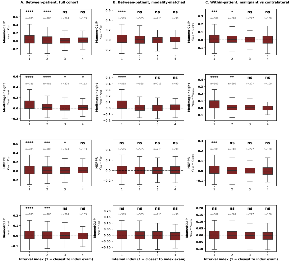
Figure 4: Per-interval paired malignant-control embedding velocity difference, breast level. (A) Between-patient (malignant case and matched control), full matched cohort. (B) Between-patient, restricted to modality-concordant pairs. (C) Within-patient (malignant biopsied and healthy contralateral breast), restricted to modality-stable patients. (A) and (B) isolate the effect of modality matching. Notably, matching on modality removes HOPPR’s significance entirely and Mammo-CLIP’s interval-2 while MedImageInsight retains significance at intervals 1 and 2. BiomedCLIP’s significance vanishes at all intervals. (C) Within-patient contralateral modality-stable analysis shows a similar pattern, but HOPPR maintains significance at interval-1, and Mammo-CLIP shows significance at both intervals 1 and 2. BiomedCLIP remains insignificant at all intervals. Positive values (above the dashed zero line) indicate faster movement toward \hat{u} . Whiskers are 1.5 \times IQR. Asterisks are the Holm-corrected per-interval paired Wilcoxon (**** p < 10^{-4} , *** p < 10^{-3} , ** p < 0.01 , * p < 0.05 ; ns = not significant); per-cell n is shown above each box.
