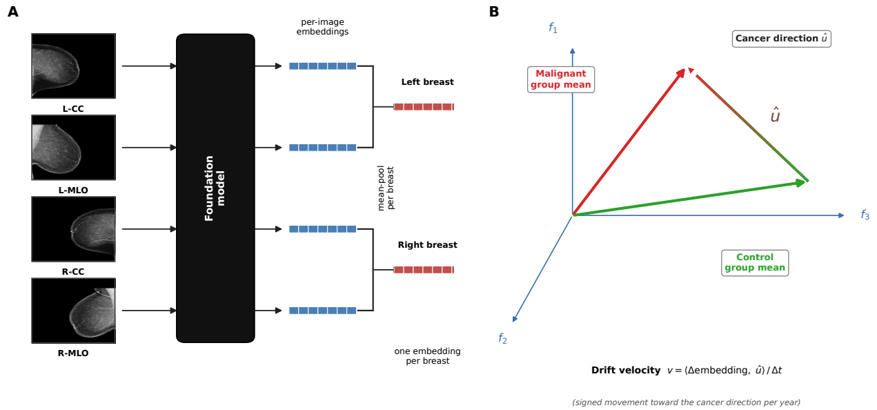
Figure 2: Embedding extraction and cancer direction definition (A) Simplified embedding extraction shown for a representative four-view screening study. Each image is passed through a frozen foundation model to produce one embedding vector per image. Image-level embeddings are mean-pooled within each breast to yield a single embedding vector per breast. An additional supplemental analysis was performed in which image-level embeddings were mean-pooled at the study level, yielding one embedding vector per study. (B) The cancer direction \hat{u} is the unit vector from the control group mean-pooled index embedding to the malignant group-mean index embedding. Directional embedding velocity v is the signed projection of an exam-to-exam embedding change onto \hat{u} per year for a given patient (§3.4–3.5).
