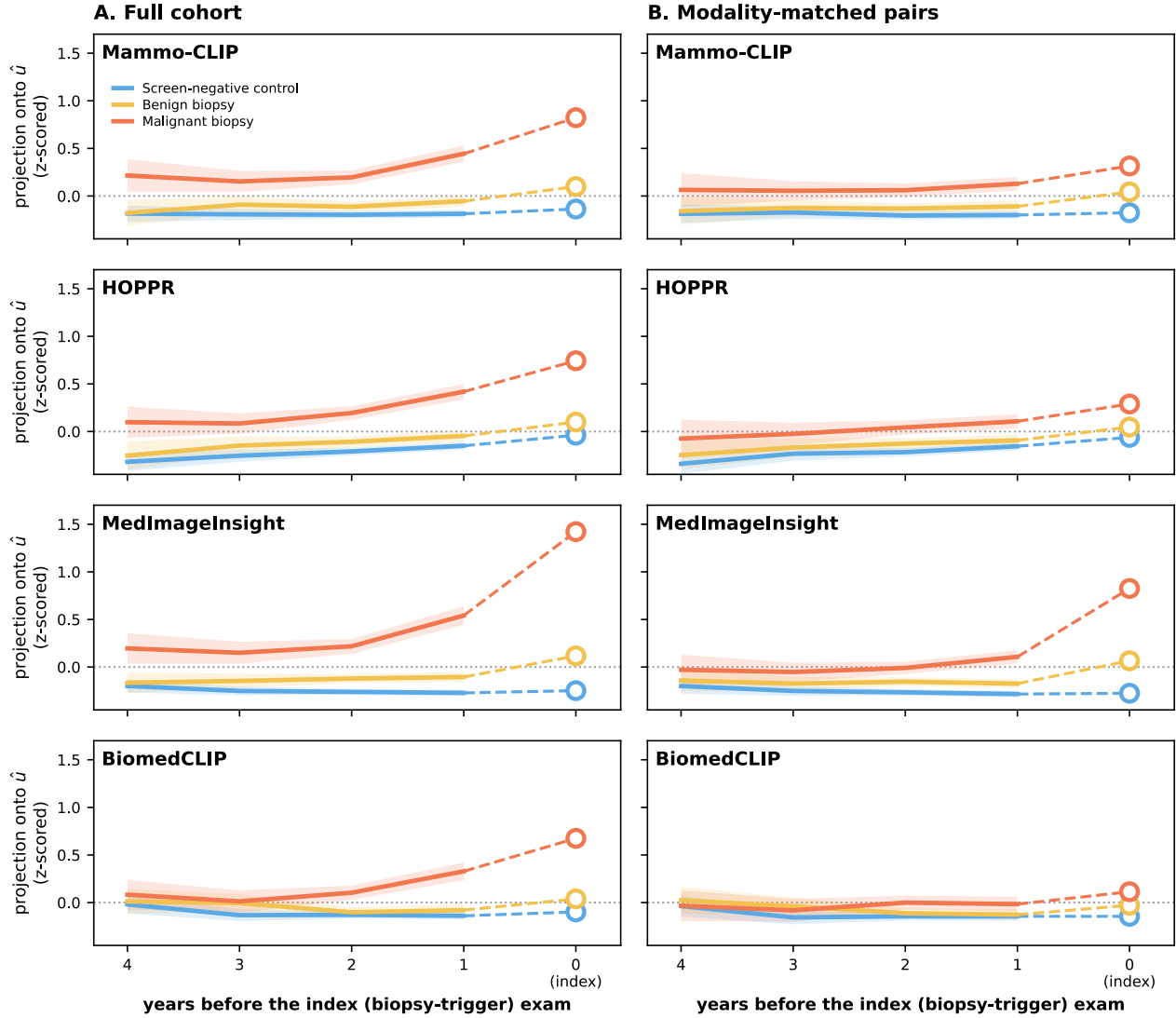
Figure 3: Group mean projection of each exam’s breast-level embedding onto the cancer direction \hat{u} . The rows, from top to bottom in each panel, represent Mammo-CLIP, HOPPR, MedImageInsight, and BiomedCLIP. (A) Full matched case-control cohort. (B) Restricted to the modality-matched pairs in which the case and control share the same modality at each interval. Here, \hat{u} is fit once on the full cohort and shared by both panels for direct comparison. Embeddings are the biopsied breast for cases and the matched control’s corresponding side. The trajectories are group means over prior exams with 95% confidence intervals. The index exam, which defines \hat{u} , is shown as open circles on a dashed segment. In (A), the malignant (orange) trajectory rises sharply toward \hat{u} at the index, while benign (yellow) and control (blue) stay flat. Under modality matching (B) the malignant rise persists for the clinical-imaging models but substantially less so for BiomedCLIP.
