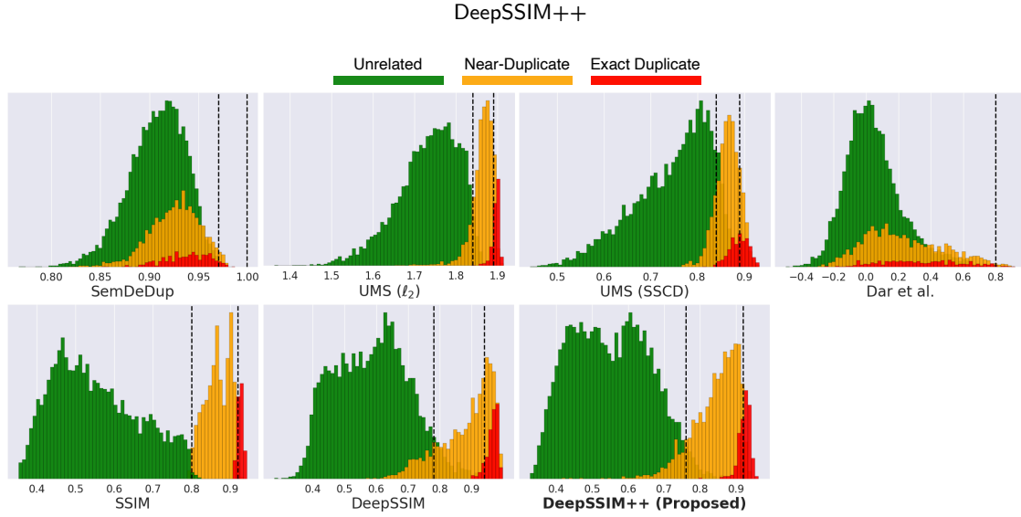
Figure 4: Similarity Score Distributions Across Methods. This figure illustrates the distribution of similarity scores predicted by each method under perfect registration, stratified by ground-truth category: Unrelated , Near-Duplicate , Exact Duplicate . Dashed vertical lines indicate the decision threshold(s) used by each method.
