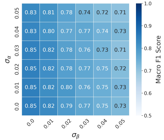
Figure 6: Sensitivity of the Proposed Thresholds. This figure illustrates the variations of the macro F1 score as a function of Gaussian noise applied to thresholds \alpha and \beta . The x- and y-axes represent increasing noise levels, corresponding to \sigma_\beta and \sigma_\alpha , respectively.
