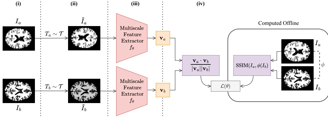
Figure 1: Training Pipeline: The figure illustrates the DeepSSIM++ self-supervised training process, which is divided as follows: (i) Inputs: real and synthetic MRI scans are first preprocessed. (ii) Augmentation: random anatomical-preserving augmentations are applied before feature extraction to improve robustness to image variability. (iii) Embeddings: images are mapped into a lower-dimensional embedding space using a feature extractor f_\theta . (iv) Model Optimization: the training loss minimizes the discrepancy between the embedding cosine similarity and the corresponding SSIM target, optimizing the feature extractor parameters \theta .
