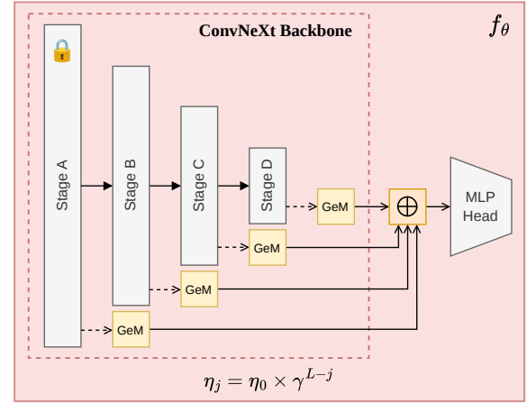
Figure 3: Feature Extractor Architecture: The figure illustrates the proposed feature extractor f_\theta , which combines a ConvNeXt backbone with multi-scale GeM pooling and an MLP-based fusion head. Feature maps are extracted from four progressively deeper stages (Stage A, B, C, and D), capturing increasingly abstract anatomical information. The stage outputs are independently pooled, concatenated, and projected into the final embedding space.
