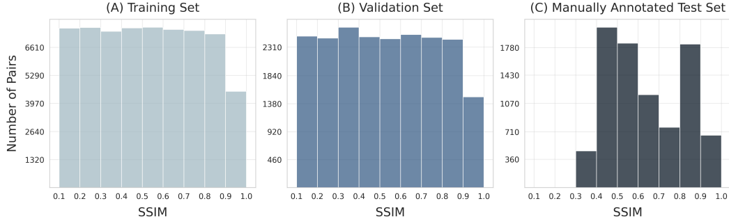
Figure 2: Distribution of Ground-Truth SSIM Scores. The figure illustrates the distribution of image pairs across SSIM bins (width 0.1) for the three dataset splits. Panels (A) and (B) show the training and validation sets, \mathcal{P}_{\text{train}} and \mathcal{P}_{\text{valid}} , respectively, both exhibiting approximately balanced distributions obtained by stratified random sampling. Panel (C) presents the manually annotated test set \mathcal{P}_{\text{test}} , which is unbalanced due to the hybrid sampling strategy.
