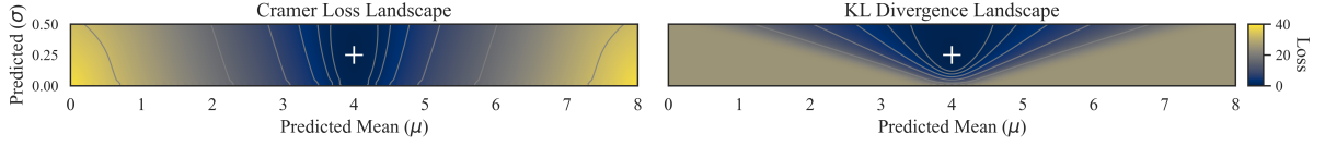
Figure 3: Comparison of the loss landscapes for the Cramér distance and KL divergence. Each heat map shows the loss as a function of the predicted mean \mu and standard deviation \sigma relative to a fixed target distribution, marked by a cross at \mu = 4.0 and \sigma = 0.25 . The Cramér distance landscape ( left ) exhibits a smooth, valley-like topology, whereas the KL-divergence landscape ( right ) is more sharply constrained. Contour levels are spaced at powers of two, with higher levels indicating greater loss.
