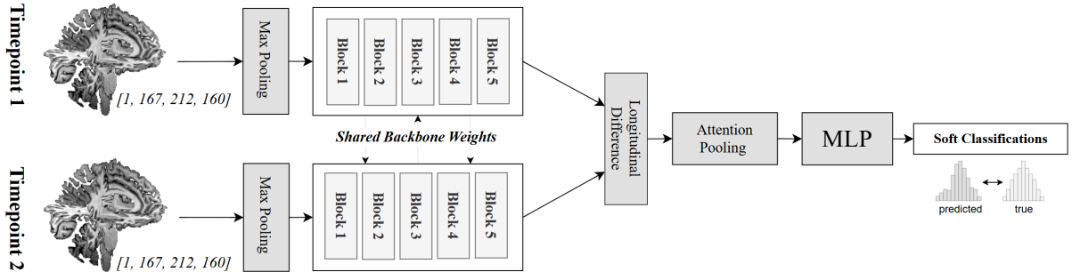
Figure 2: Proposed Siamese deep learning architecture for longitudinal brain age estimation. Longitudinal T1-weighted image pairs (Timepoint 1 and Timepoint 2) are processed through a shared SFCN-style backbone. Resulting timepoint-specific feature vectors are fused via subtraction. The difference vector is then passed to the spatial attention pooling module and Multi-Layer Perceptron head to finally produce a soft classification distribution.
