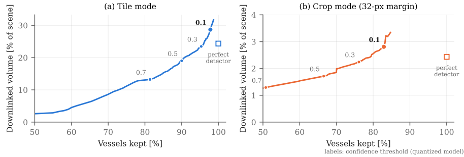
Fig. 5. Downlinked volume versus vessels kept, quantized detector, confidence threshold swept (labels; large dot: 0.10, used in Table 7): (a) tile mode, (b) crop mode. Squares: perfect detector.
