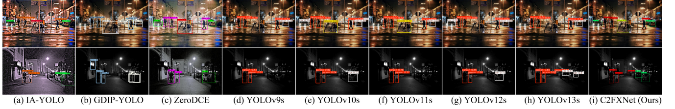
Figure 6: Visual comparison on the ExDark dataset under low-light conditions. C2FXNet achieves more accurate and confident detections, successfully identifying objects in dark and overexposed areas.
