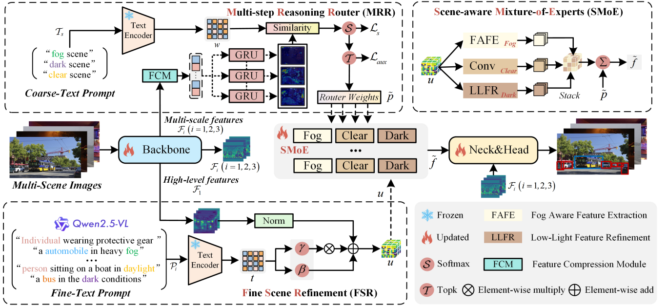
Figure 2: Overview of proposed C2FXNet. It consists of three key modules: the Multi-step Reasoning Router (MRR) compresses multi-scale visual cues and performs GRU-based recurrent scene reasoning under coarse text-guided prototypes to generate interpretable routing weights, the Fine Scene Refinement (FSR) refines visual features using fine-grained textual cues, and the Scene-aware Mixture-of-Experts (SMoE) dynamically fuses fog, dark, and clear experts under the joint guidance of MRR and FSR, enabling robust and scene-consistent detection. Among them, \gamma and \beta denote two learnable linear layers.
