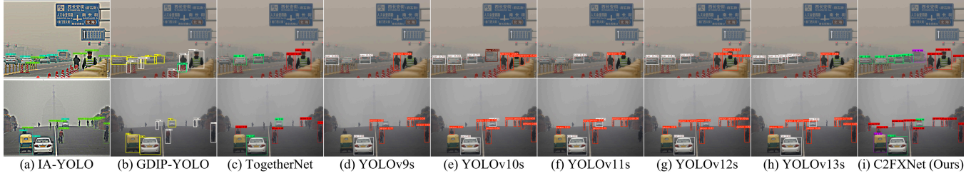
Figure 5: Visual comparison on the RTTS dataset under foggy conditions. C2FXNet detects more objects with clearer boundaries and higher confidence, especially for small or distant targets that other methods miss.
