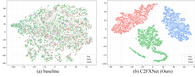
Figure 4: t-SNE visualization of feature embeddings. C2FXNet produces more compact and better-separated clusters than the baseline for fog, dark, and clear scenes.
