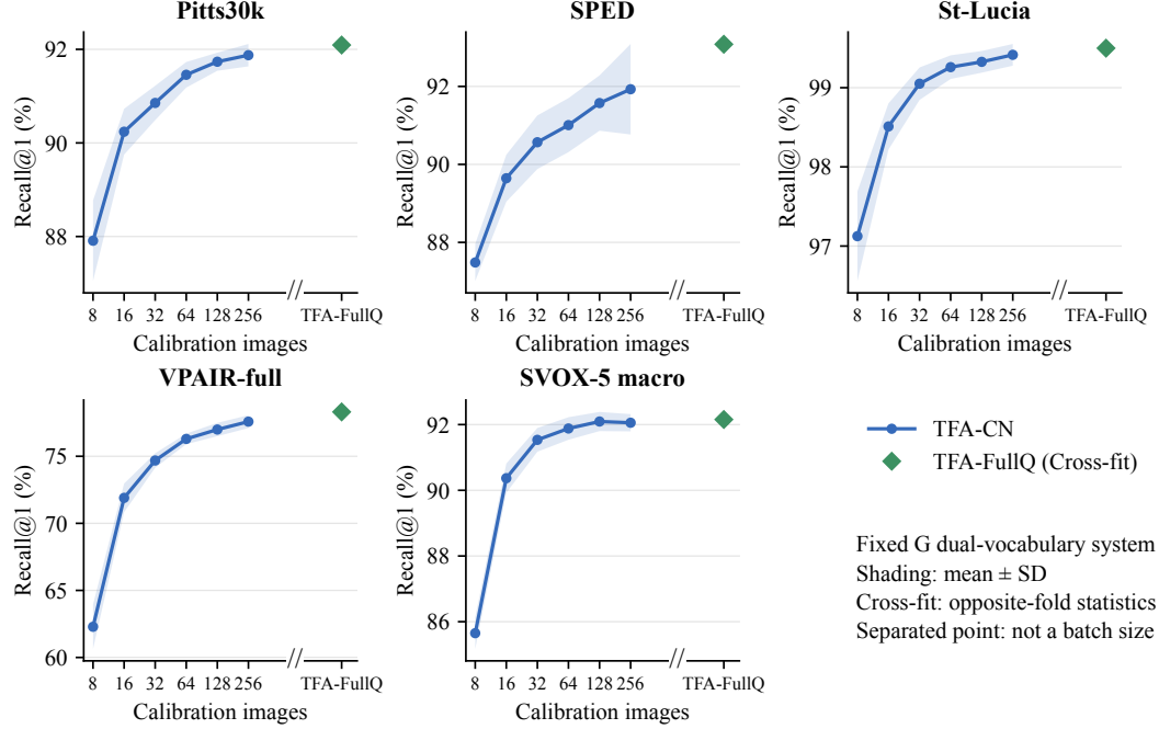
Figure 3: Disjoint calibration-size experiment, R@1. Blue: DINOv2-G dual-vocabulary TFA-CN system, mean±SD over ten splits. The separated TFA-FullQ (Cross-fit) point uses opposite-fold query statistics (Table 3); its horizontal position is schematic. All points use the same backbone and dual-vocabulary configuration; calibration and evaluation sets follow the stated protocols.
