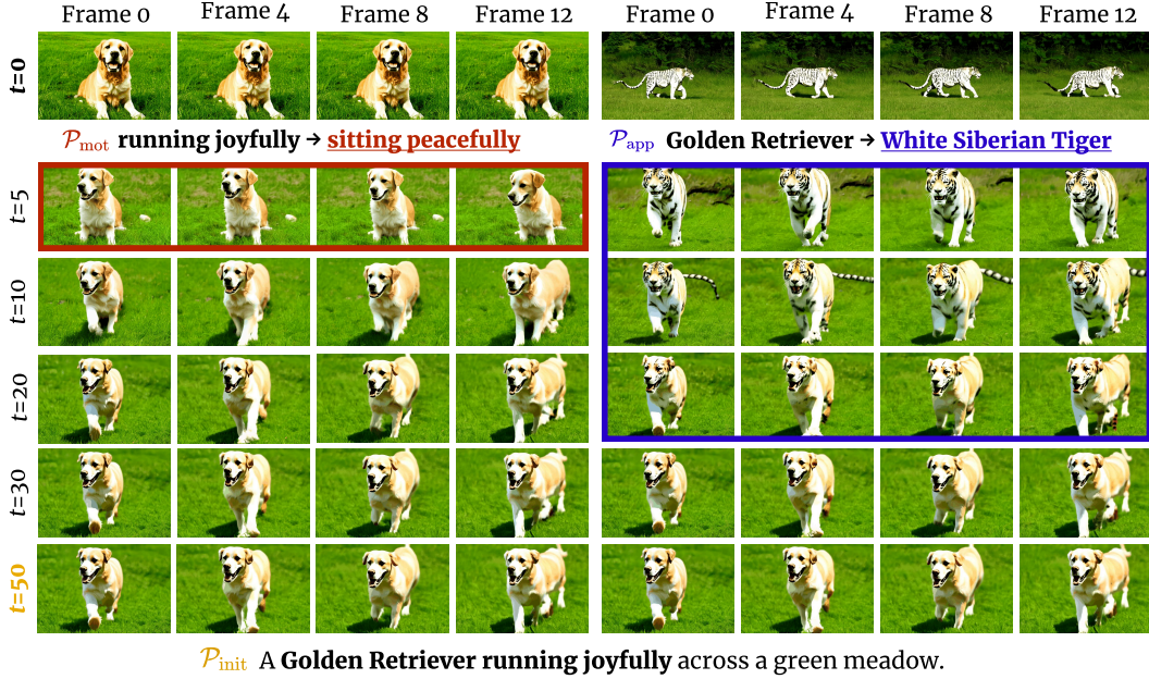
Figure 3: Qualitative analysis on motion formation timestep. The y -axis indicates the switching timestep ( t \in [0, 50] ) at which the initial prompt \mathcal{P}_{\text{init}} is switched to a new prompt \mathcal{P}_{\text{mot}} or \mathcal{P}_{\text{app}} . Left: Switching from \mathcal{P}_{\text{init}} to \mathcal{P}_{\text{mot}} shows that motion becomes largely established after early timesteps ( t = 10 ), with limited influence from subsequent prompts. Right: Switching to \mathcal{P}_{\text{app}} shows that non-motion can still change at later timestep ( t = 20 ).
