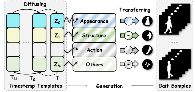
Figure 1. Origins performs unified generative and representation learning. The unified template \mathcal{T} diffuses to the timestep templates, which generates gait representations. Meanwhile, the unified template \mathcal{T} transfers to capture accurate gait differences.
