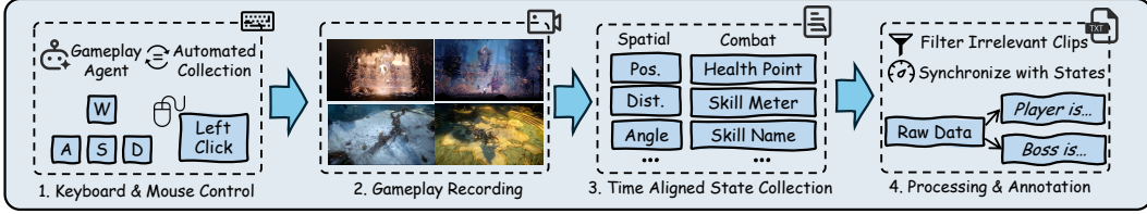
Figure 2: Data Collection Pipeline. An automated gameplay agent collects keyboard and mouse inputs, gameplay recordings, and temporally aligned state information across three games, followed by filtering, synchronization, and annotation to construct the final dataset.
