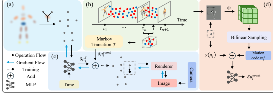
Figure 1: Overview of EdMCGS. (a) We initialize the control points by sampling from the canonical space. (b) We cast the deformation as an event-driven Markov chain, where the events accumulated in the interval [\tau_n, t] between two RGB anchors drive a Markov transition of the control point state. (c) At a query time t , the coarse RGB-driven deformation predicted by the MLP and the fine event-driven correction from the Markov transition are added to displace the control points, which in turn deform the Gaussians by linear-blend skinning before rasterization. (d) Local event sampling: the events in [\tau_n, t] are accumulated into a polarity map, encoded by a shallow CNN \Phi , and bilingually sampled at each control point’s projection to form its local motion code.
