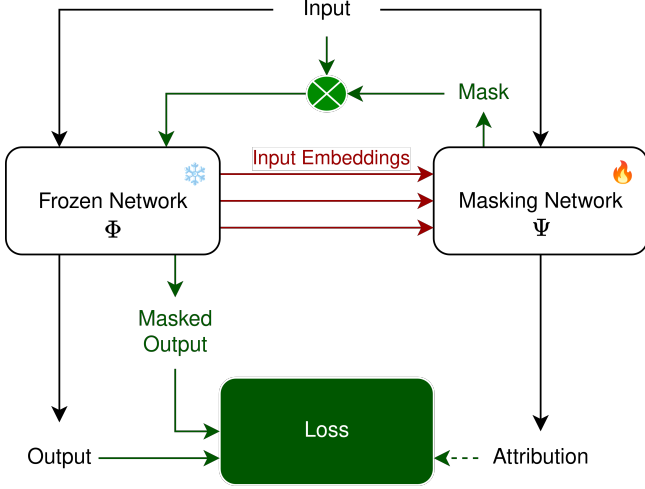
Fig. 1. The general Neural Explanation Method (NEM) framework’s operation during inference (black and red arrows) and training (black, red, and green arrows). During inference, the input is processed by the frozen network, which generates its output, and the masking network, which produces an attribution (explanation). Depending on the NEM architecture, representations from the frozen network may assist the masking network in generating the attribution. During training, the masking network generates a mask from the attribution. In [10], [11], this mapping is the identity, and in this work it is a differentiable top- k feature selector. The mask is applied to the input and passed through the frozen network to produce a masked output. Both masked and unmasked outputs are used in a loss function to optimize the masking network. Prior work has also incorporated the attribution into the loss.
