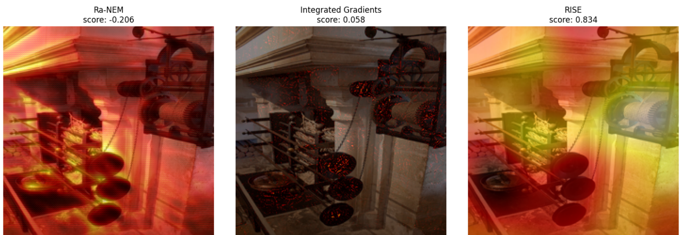
Fig. 20. Example of image from ImageNet test set, where Ra-NEM performs relatively poor compared to other methods. Score is Faithfulness. We include Integrated Gradients and RISE for comparison. The explained model is a ResNet50 trained on the training split of the ImageNet dataset. Here Ra-NEM predicts that the wrong object is the most important.
