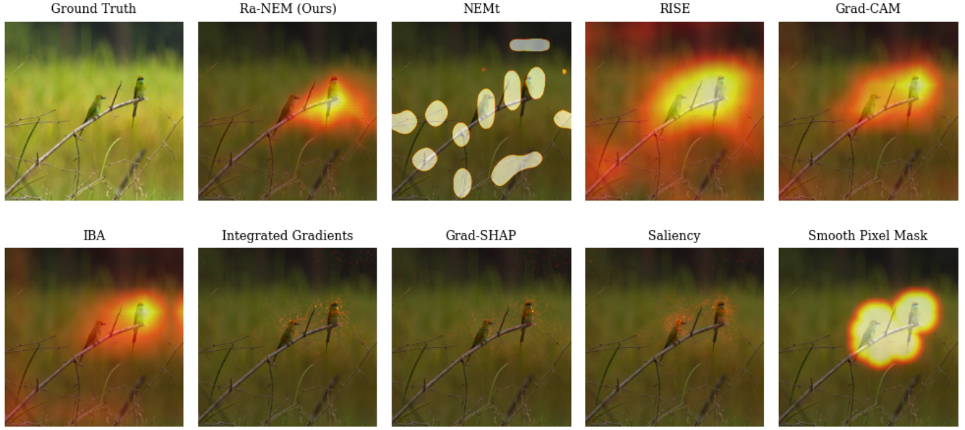
Fig. 10. Model explanations generated by different XAI methodologies. The explained model is a VGG16 architecture trained on the training split of the ImageNet dataset. The example image is taken from the validation split of the ImageNet dataset.
