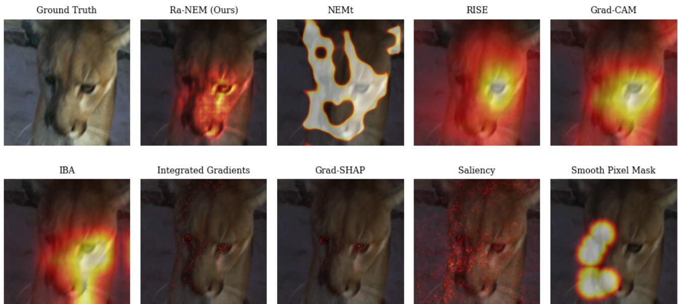
Fig. 3. Model explanations generated by various different XAI methodologies. The explained model is a ResNet50 architecture trained on the training split of the ImageNet dataset. The example image is taken from the validation split of the ImageNet dataset. Comparing Ra-NEM with other occlusion-based methods, we observe that its finer granularity more precisely reveals specific image features. While all methods highlight the importance of the eye, Ra-NEM identifies only a small region of the eye and its outline as necessary.
