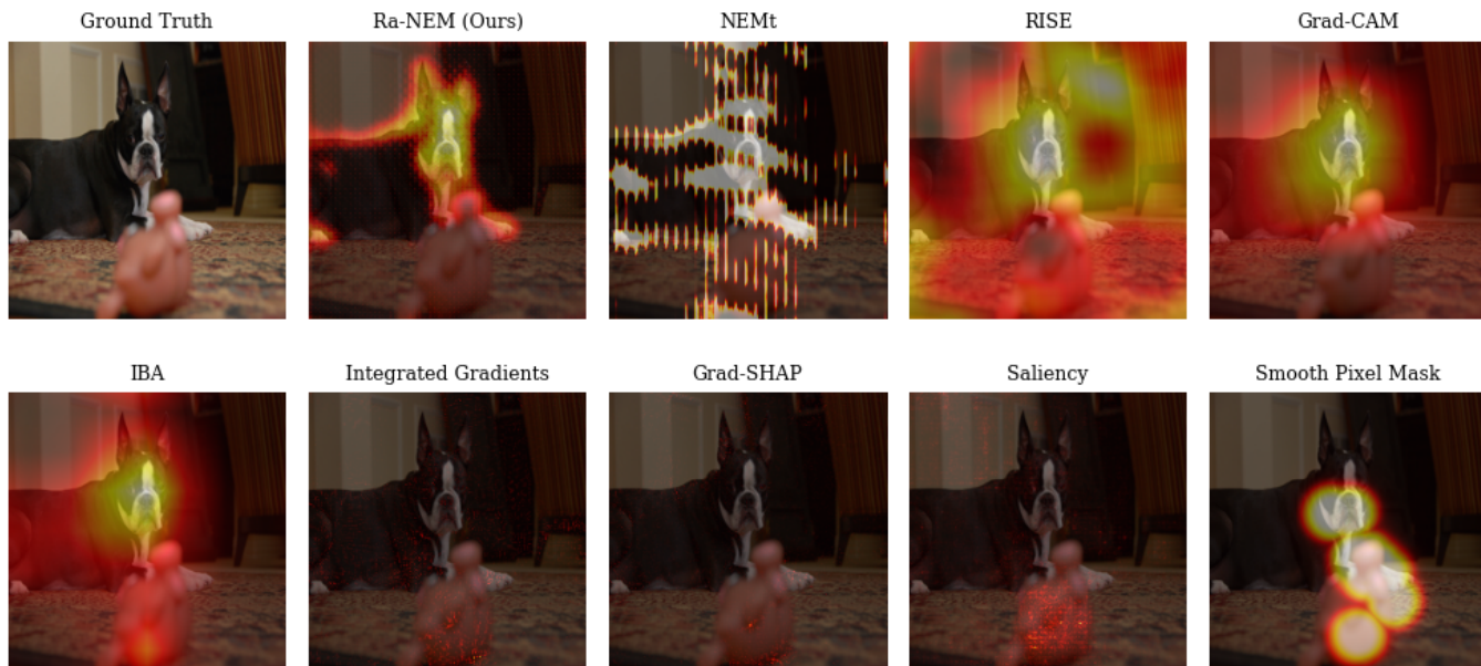
Fig. 6. Model explanations generated by different XAI methodologies. The explained model is a ConvNeXt architecture trained on the training split of the ImageNet dataset. The example image is taken from the validation split of the ImageNet dataset. It can be seen that all occlusion-based methods agree that the face of the dog is important, but Ra-NEM also emphasizes the ears.
