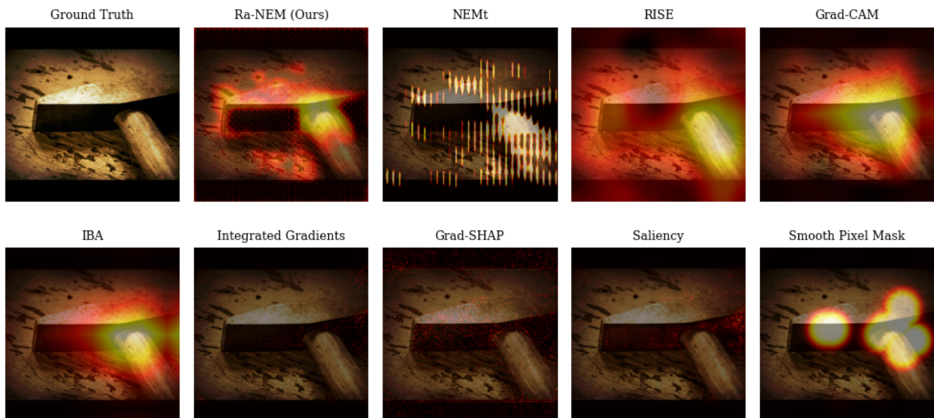
Fig. 5. Model explanations generated by different XAI methodologies. The explained model is a ConvNeXt architecture trained on the training split of the ImageNet dataset. The example image is taken from the validation split of the ImageNet dataset. Occlusion-based methods generally agree on the area of interest, but only Ra-NEM with its high granularity can outline specific features. For example, it highlights both the shaft of the hammer and the outline of the hammerhead, which indicates that most of the hammerhead is not needed for classification.
