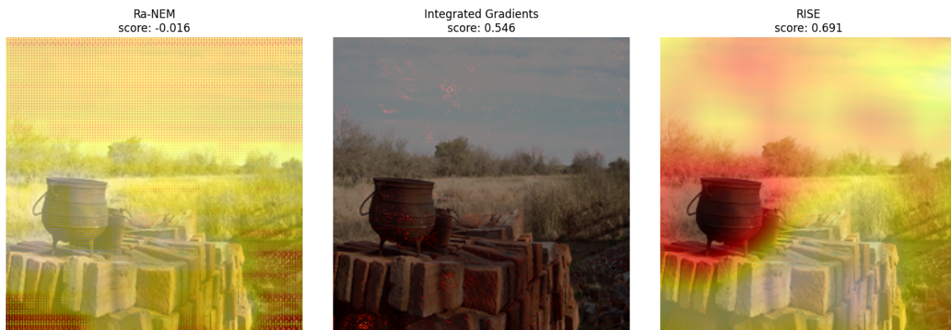
Fig. 15. Example of image from ImageNet test set, where Ra-NEM performs relatively poor compared to other methods. Score is Faithfulness. We include Integrated Gradients and RISE for comparison. The explained model is a ConvNeXt trained on the trainings split of the ImageNet dataset.
