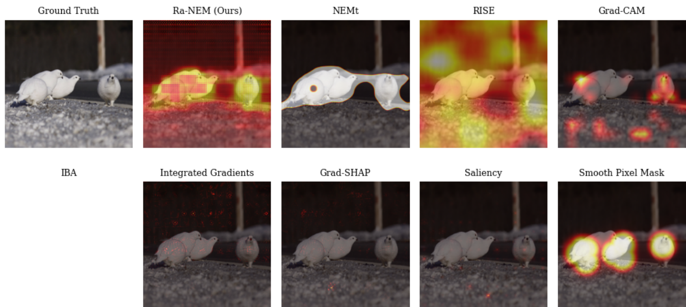
Fig. 13. Model explanations generated by different XAI methodologies. The explained model is a ViT architecture trained on the training split of the ImageNet dataset. The example image is taken from the validation split of the ImageNet dataset. As there is no adaptation of IBA for transformer-based image models, IBA results have not been generated. This example underpins many of the points already discussed in Figure 11, a.i. the confusion of methods leveraging smoothing and the limited interpretability of Integrated Gradients, despite its higher faithfulness score. Additionally, NEMt occasionally generates very large attributions for the ViT.
