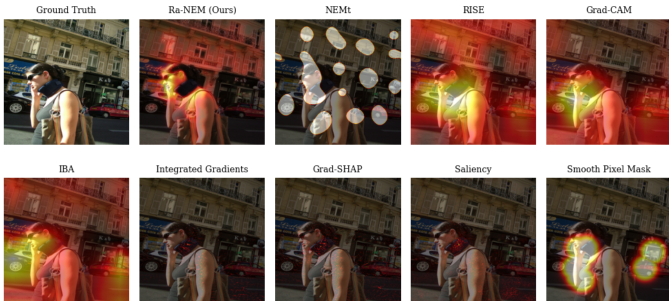
Fig. 8. Model explanations generated by different XAI methodologies. The explained model is a VGG16 architecture trained on the training split of the ImageNet dataset. The example image is taken from the validation split of the ImageNet dataset. Notably, Ra-NEM excludes the neck brace, whereas the smoothing of the other occlusion based methods somewhat include it as an important feature. Furthermore, it can be seen that the gradient based methods all generally target the neck brace.
