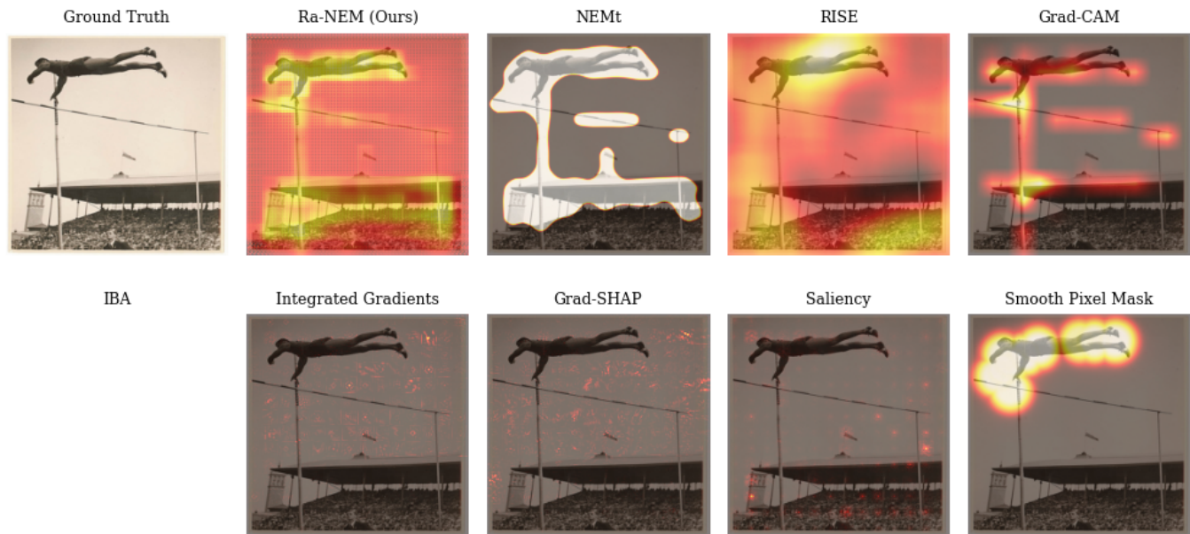
Fig. 12. Model explanations generated by different XAI methodologies. The explained model is a ViT architecture trained on the training split of the ImageNet dataset. The example image is taken from the validation split of the ImageNet dataset. There is no adaptation of IBA for transformer-based image models, so IBA results have not been generated.
