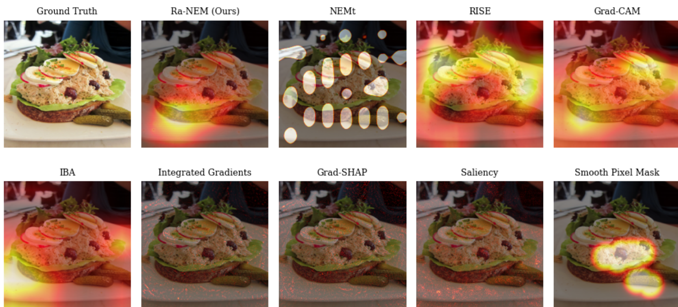
Fig. 9. Model explanations generated by different XAI methodologies. The explained model is a VGG16 architecture trained on the training split of the ImageNet dataset. The example image is taken from the validation split of the ImageNet dataset.
