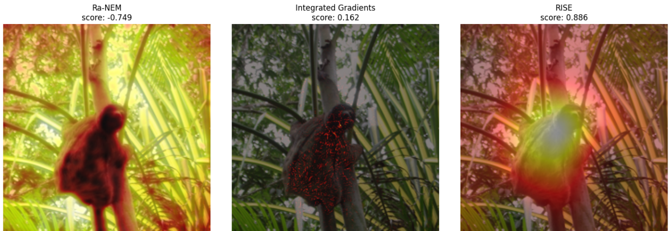
Fig. 19. Example of image from ImageNet test set, where Ra-NEM performs relatively poor compared to other methods. Score is Faithfulness. We include Integrated Gradients and RISE for comparison. The explained model is a VGG16 trained on the training split of the ImageNet dataset. Here it can be seen, that Ra-NEM has again switched foreground for background.
