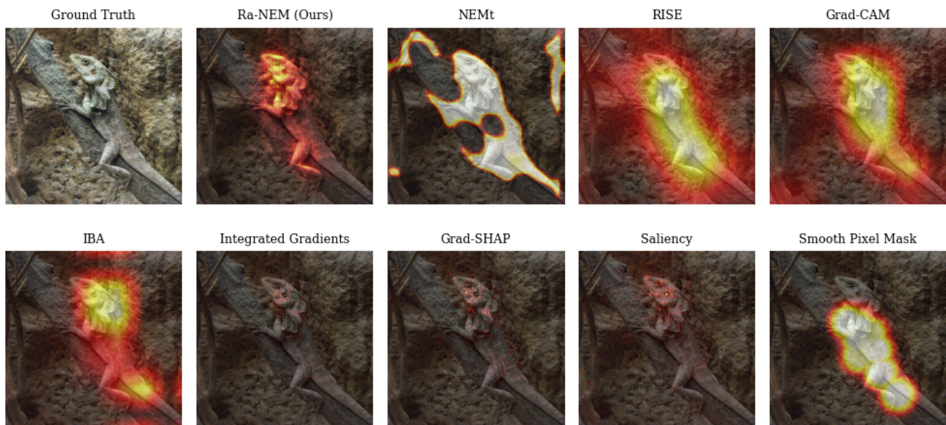
Fig. 4. Model explanations generated by various different XAI methodologies. The explained model is a ResNet50 architecture trained on the training split of the ImageNet dataset. The example image is taken from the validation split of the ImageNet dataset.
