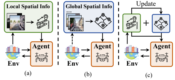
Figure 1: Comparison of three spatial representation paradigms in zero-shot methods: (a) the local-centric paradigm, (b) the global-centric paradigm, and (c) our anchor-centric paradigm, which bridges spatial information across both scales.
