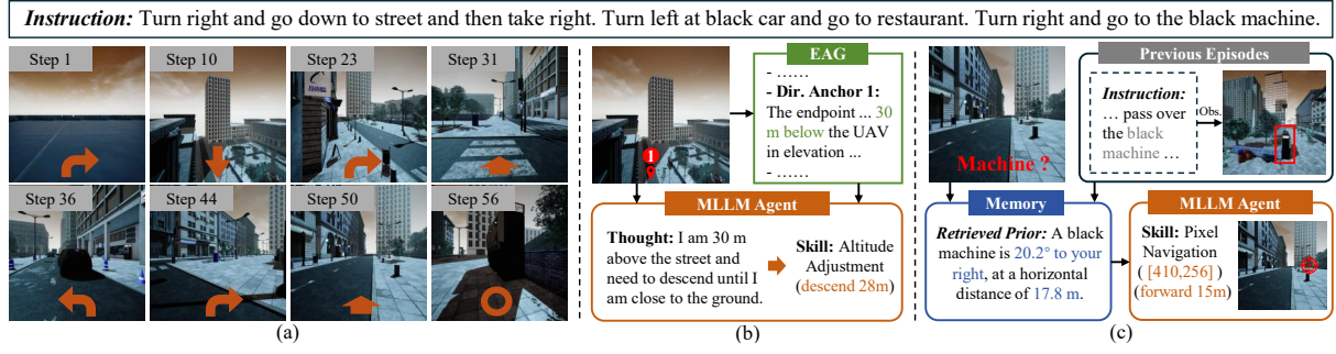
Figure 5: Visualization of a successful navigation episode. (a) Key steps throughout the episode. (b) Local spatial grounding at Step 10. (c) Global prior guidance at Step 50.
