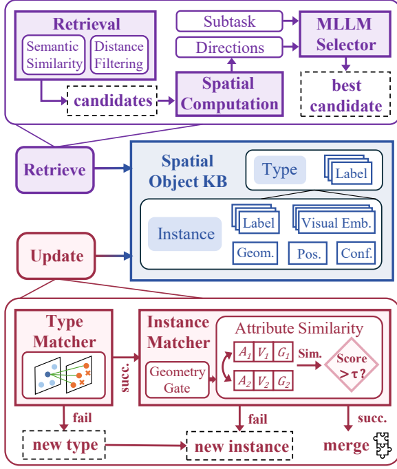
Figure 3: Overview of Persistent Object Spatial Memory. Centered on the SOKB, it maintains the global spatial representation to support reliable landmark-prior retrieval and online object knowledge updates.
