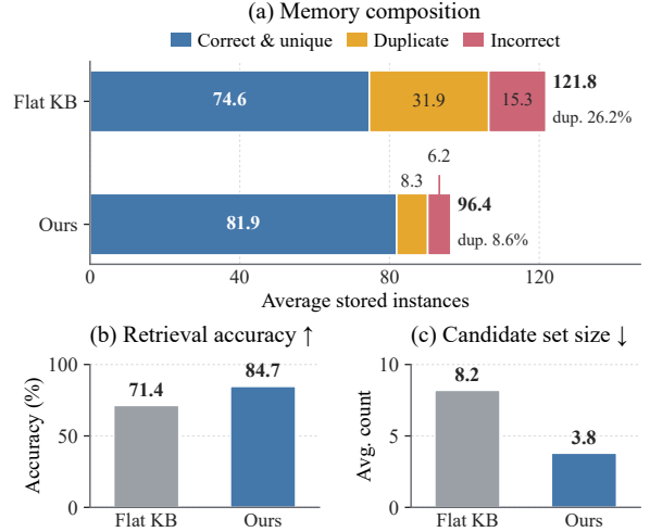
Figure 4: Comparison of object knowledge base design. We compare the proposed SOKB with a flat KB in terms of (a) memory composition, (b) landmark retrieval accuracy, and (c) candidate-set size.
