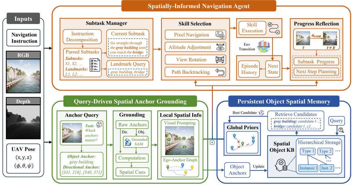
Figure 2: AirAnchor consists of three key modules. Query-Driven Spatial Anchor Grounding identifies spatial anchors and constructs the local spatial representation. Persistent Object Spatial Memory maintains the global spatial representation, supporting online updates and prior knowledge retrieval. Spatially-Informed Navigation Agent integrates the local spatial representation and global spatial priors within an agentic framework to enable closed-loop and spatially grounded navigation decisions.
