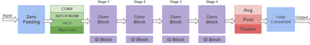
Figure 1: ResNet50 architecture overview comprising zero padding, four residual stages, average pooling, and fully connected output layer. Source: Author, based on (Mukherjee, 2022).
