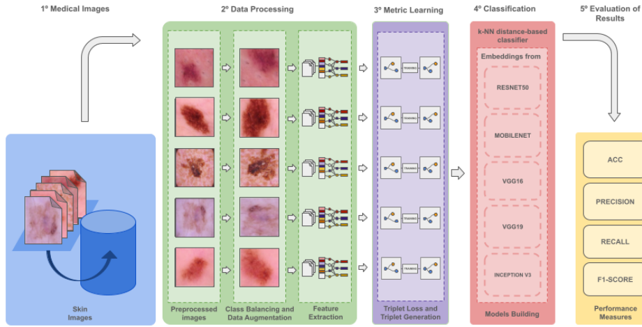
Figure 5: Overall workflow of the proposed method. In the case of the CR-AI4SKIN dataset, pre-computed embeddings were directly used in the classification stage, and the image processing and metric learning steps were not applied.
