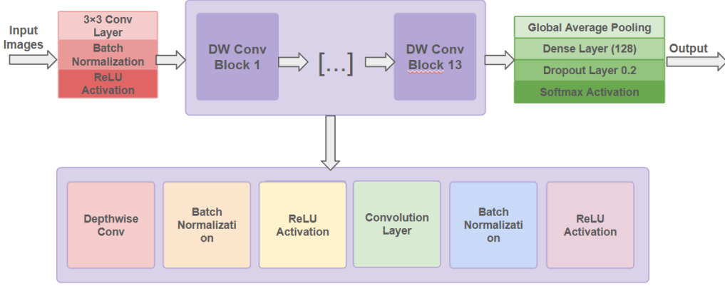
Figure 2: MobileNet architecture overview comprising an initial convolution block, 13 depthwise separable convolution blocks, global average pooling, and softmax output. Source: elaborated by the author based on (Asif et al., 2024).
