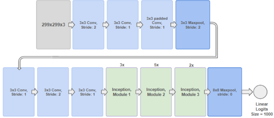
Figure 4: InceptionV3 architecture overview comprising initial convolution stages, three inception module groups, and a linear output layer. Source: elaborated by the author based on (Asif et al., 2024).
