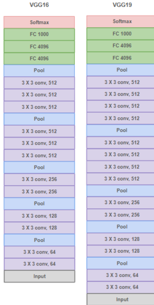
Figure 3: VGG16 and VGG19 architecture overview comprising stacked 3 \times 3 convolutional layers, max-pooling stages, and fully connected layers with softmax output. Source: elaborated by the author based on ( datahacker.rs , 2018).
