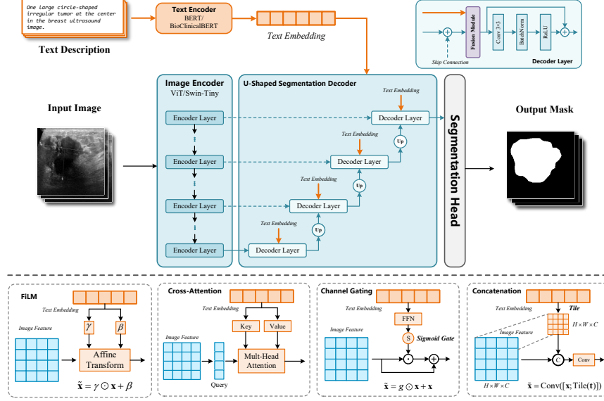
Fig. 1. Our baseline framework feeds image samples and corresponding text into the image encoder and text encoder, respectively. The resulting features are then processed step by step through a U-shaped segmentation decoder for segmentation. The lower half of the figure provides a schematic of the four fusion operators.
