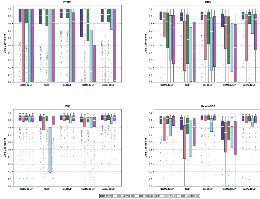
Fig. 3. Box plots of the Dice metric for five models tested on four datasets with text perturbations.
