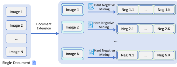
Figure 2: Process of creating DocLongRAG.
