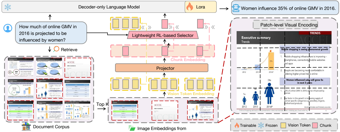
Figure 3: Architecture of Doc-REFRAG. Retrieved document images are encoded patch-level into chunk embeddings. A query-aware RL-based selector identifies informative chunks, which are expanded to fine-grained tokens before being fed with the query into a decoder-only language model.
