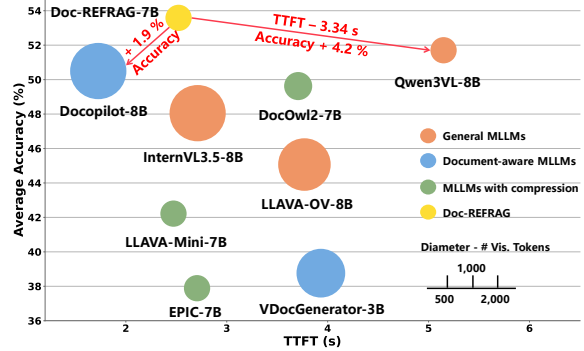
Figure 1: Doc-REFRAG achieves the best accuracy-efficiency trade-off among MLLMs.
