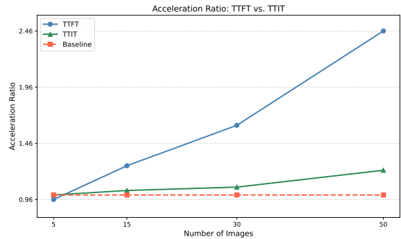
Figure 7: Acceleration ratio of Doc-REFRAG versus DocOwl2 in terms of TTFT (blue) and TTIT (green), as a function of the number of retrieved images. The red dashed line indicates the baseline (DocOwl2 Latency = 1\times ).
