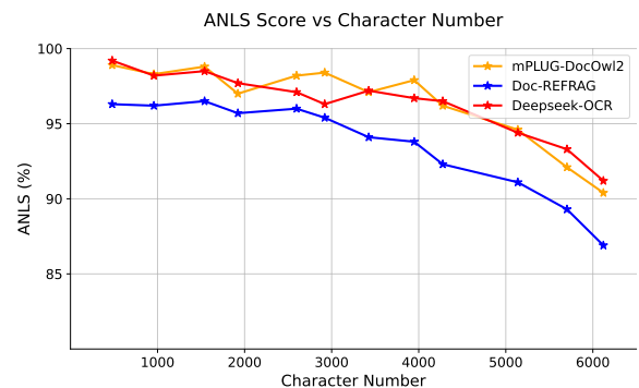
Figure 4: Parsing performance on A4 document image.
