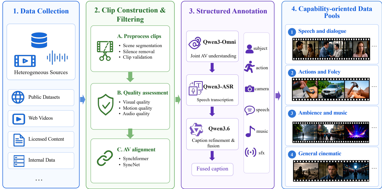
Figure 3 Overview of the data system for DreamX-Creator 1.0, including heterogeneous data collection, clip construction and filtering, structured multimodal annotation, and capability-oriented data organization.
