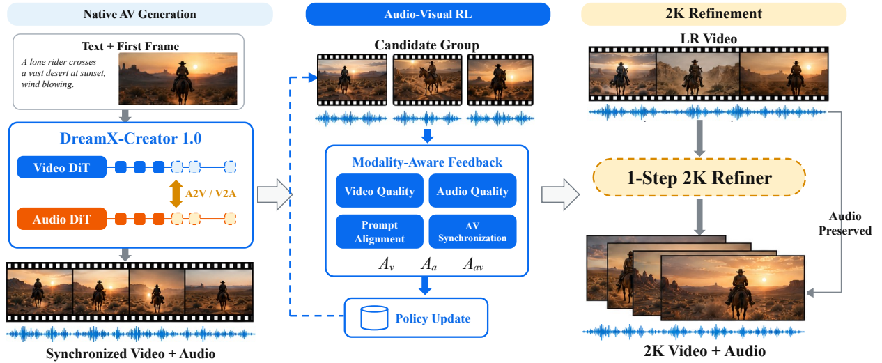
Figure 2 The DreamX-Creator 1.0 pipeline, comprising native joint audio-video generation, Audio-Video Reinforcement Learning post-training, and Autoregressive 1-Step 2K Refinement.
