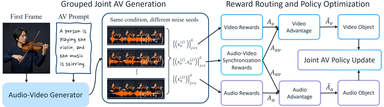
Figure 6 Modality-aware reinforcement learning for joint audio-video generation. Video- and audio-specific rewards are routed to their corresponding streams, while the shared audio-visual synchronization reward jointly optimizes both streams and their cross-modal interactions.
