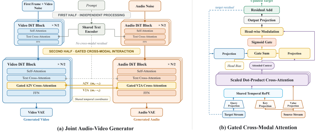
Figure 5 Architecture of the joint audio-video generator. The two streams are processed independently in the first half and interact through gated A2V and V2A cross-attention in the latter half.
