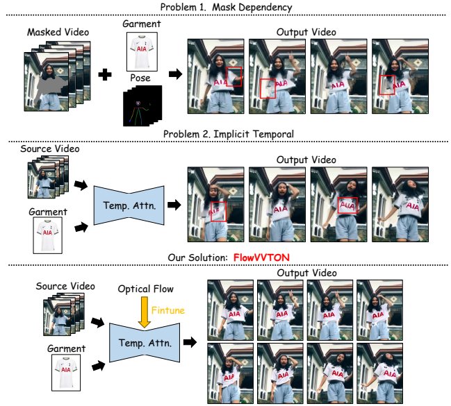
Figure 1: FlowVVTON performs mask-free video virtual try-on. Given only a source video and a target garment image, our method generates temporally consistent try-on results across all frames without any human parsing masks, pose keypoints, or region annotations. Temporal consistency is enforced during training via a flow-warped latent loss applied across all layers of the generation model.
