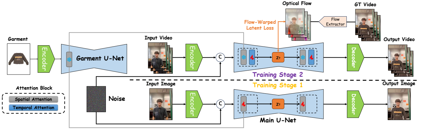
Figure 2: Overview of FlowVVTON. A reference UNet extracts garment features and injects them into the main UNet via mutual self-attention. The main UNet with temporal attention generates video frames from concatenated noisy and source latents. At every layer of the main UNet, a flow-warped latent loss enforces temporal consistency by aligning features across adjacent frames under optical flow guidance.
