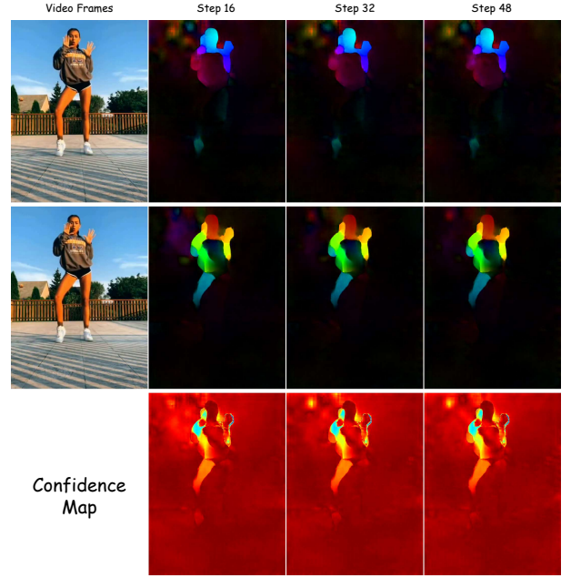
Figure 8: Flow quality analysis. The flow field at 16 iterations shows visible noise and misalignment at motion boundaries, while the 32-iteration result is substantially cleaner. The 48-iteration flow is nearly indistinguishable from 32, confirming diminishing returns.
