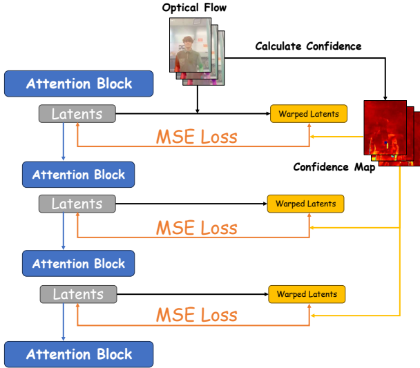
Figure 3: Detail of the flow-warped latent loss. Optical flow is computed between adjacent frames and downsampled to each layer. At every layer, the main UNet’s clean features from frame t+1 are warped backward via optical flow and compared with frame t ’s clean features via MSE loss. Confidence weights from forward-backward consistency suppress unreliable flow regions.
