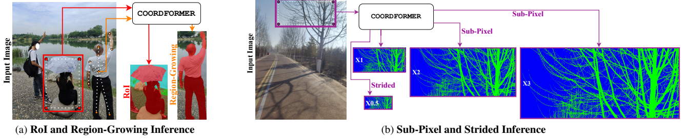
Figure A2. Inference protocols enabled by COORDFORMER. Beyond the Semantic-Edge-Focused Inference described in the main paper, COORDFORMER supports several other inference protocols: RoI querying, region growing, sub-pixel, and strided inference.
