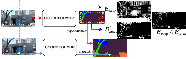
Figure 3. Semantic-Edge-Focused Inference Overview
