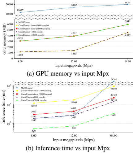
Figure 5. GPU Memory footprint (a) and Inference Times (b) of COORDFORMER, COORDFORMER dense (no SEFI) and MaSSFormer. GPU memory footprint (a) and inference time (b) are evaluated at input resolutions of 8, 12, and 64 Mpx, with COORDFORMER tested using coordinate batch of 1k and 50k.
