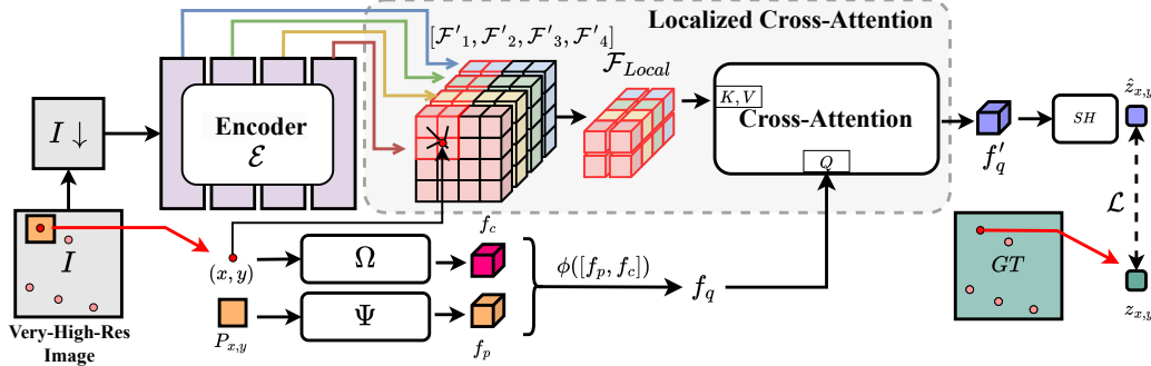
Figure 2. COORDFORMER Architecture and Training Overview. Given a very-high-resolution image ( > 4\text{Mpx} ), a ViT-based foundation encoder, \mathcal{E} , extracts globally contextualized tokens from a downsampled input, while a Coordinate Decoder builds coordinate-aware query features, f_q , from local high-resolution patches, P_{x,y} , and pixel coordinates, (x, y) . These queries interact with nearby global tokens through Localized Cross-Attention obtaining features, f'_q rich in both semantics and fine-details. These are passed to a Segmentation Head (SH) to predict class logits, \hat{z}_{x,y} , at the queried locations. During training, pixel and label information is sampled from random coordinates of images and ground truths, and the network is optimized with multi-class Cross-entropy, per-class Dice and per-class Cross-entropy losses.
