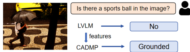
(a) The grounded samples detected by CADMP on POPE
