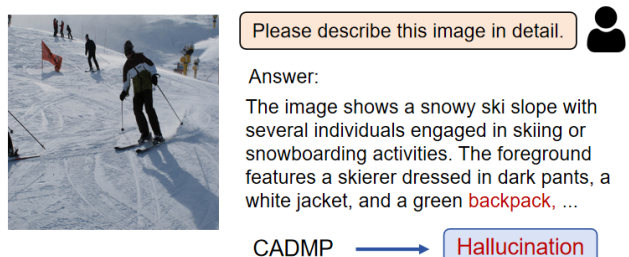
(c) The grounded and hallucination samples detected by CADMP on MSCOCO
